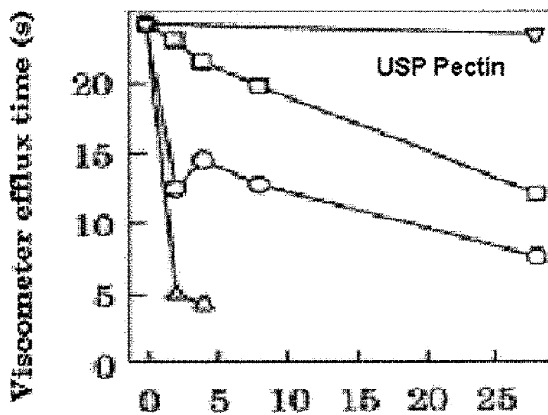
Figure 1 Scission of polysaccharides by ascorbate and/or H 2 O 2 The effect of 10 mM H 2 O 2 (□), 10 mM ascorbate (○), or 5 mM of each (△)
