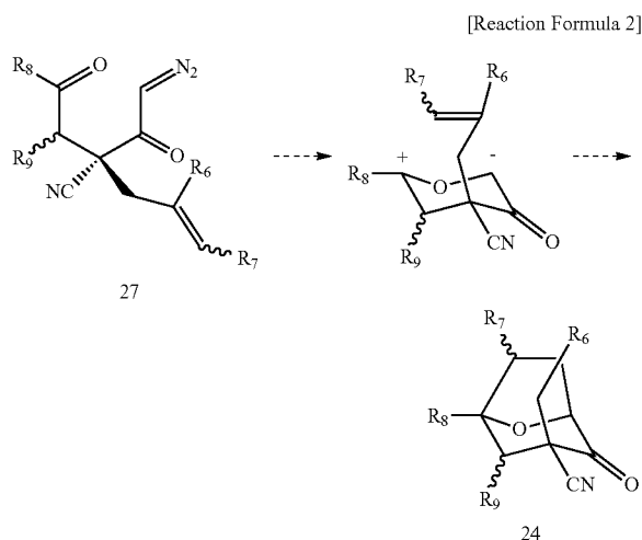
[Reaction Formula 2]
