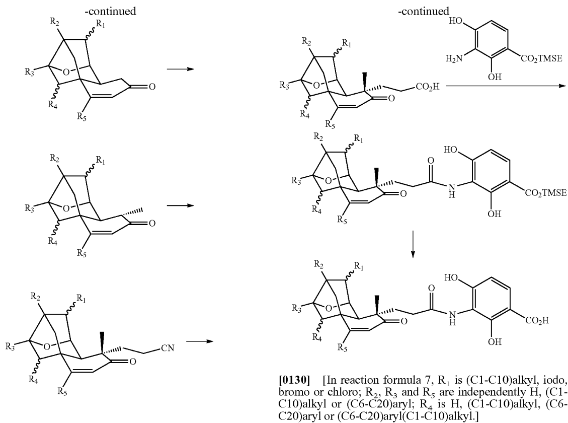
[Reaction Formula 8]
