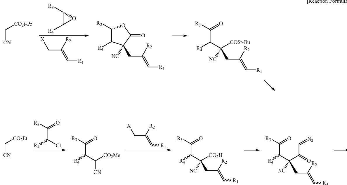
[Reaction Formula 8]
