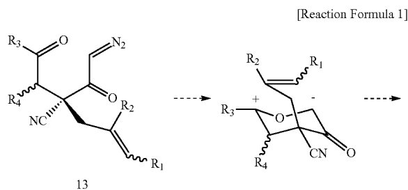
[Reaction Formula 1]
