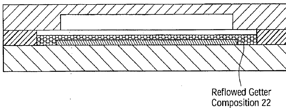
Encapsulated Device After Reflow Of Getter 20
