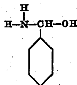
Benzylol amine
