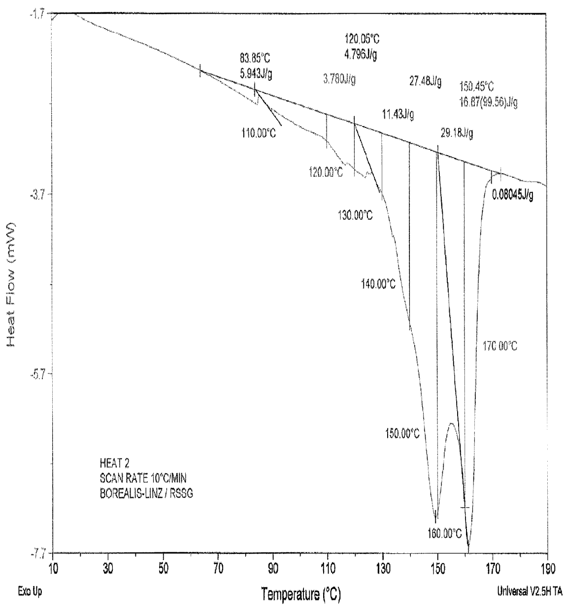
SIST Curve E 1 (6.76 mg sample)
