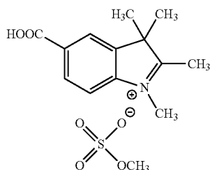
Synthesis Example 20
