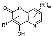
4-hydroxy-4a,8a-dihydro-pyrano[3,2,b]pyridin-2-one
