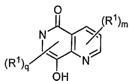
8-hydroxy-6H-[1,6]naphthyridin-5-one
