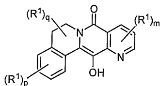
dibenzo[a,g]quinolizin-8-one
