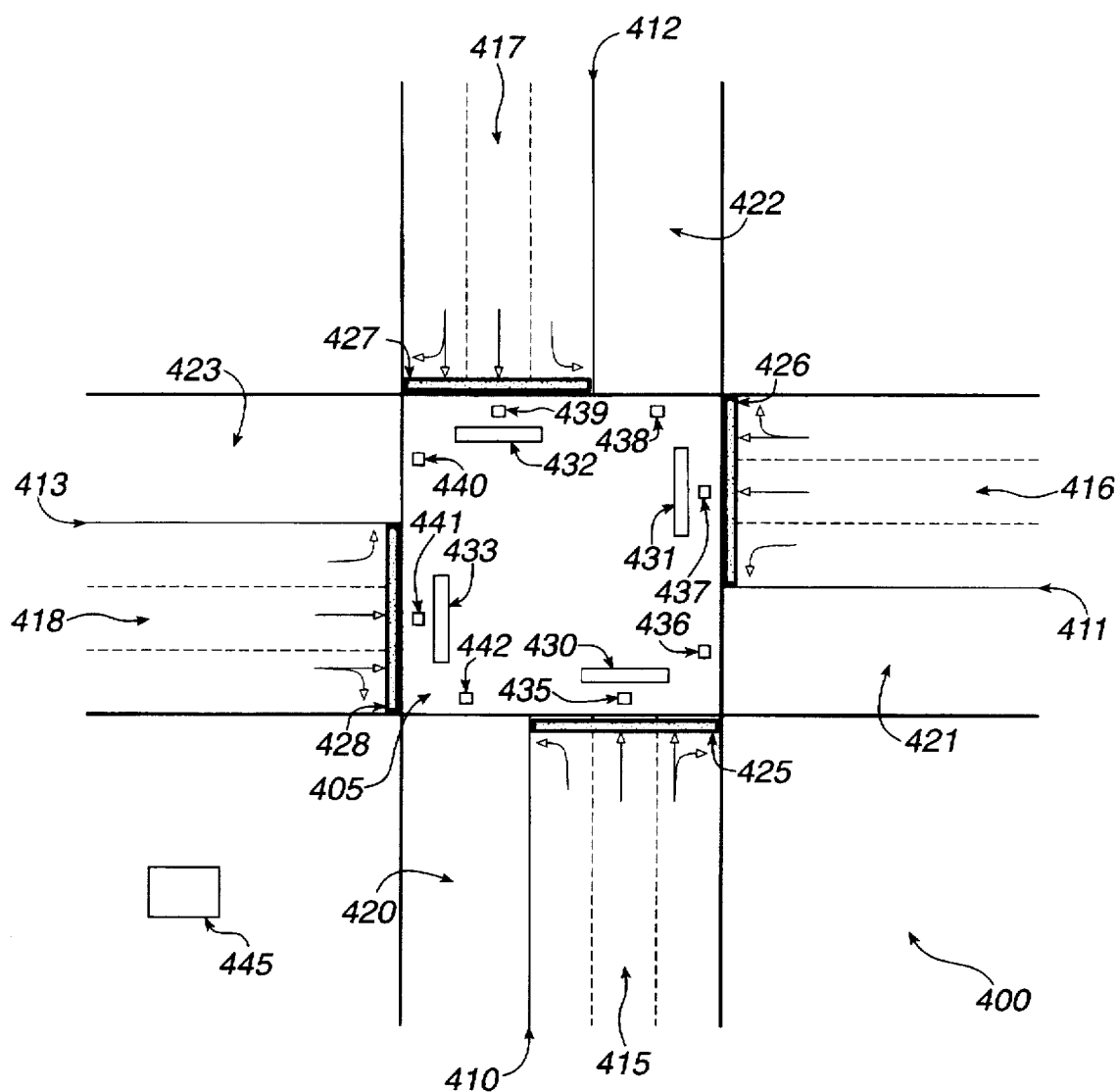
Preferred Embodiment of System for Controlling Movement of Vehicles Through an Intersection
