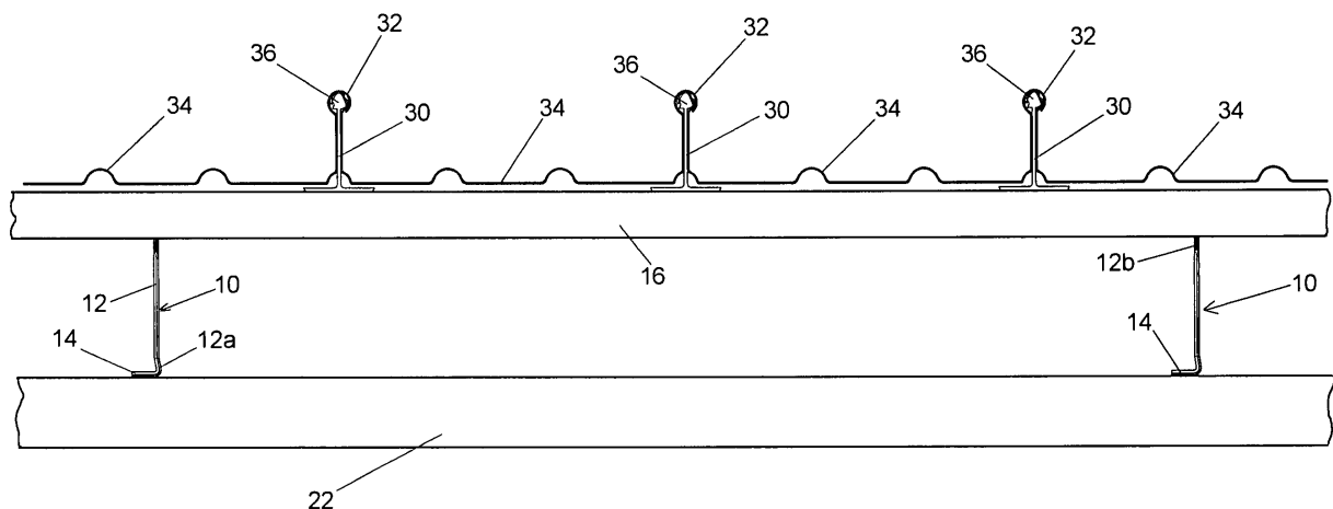
Fig 1. (PRIOR ART)
