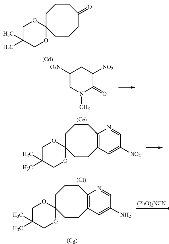
REACTION SCHEME 4
