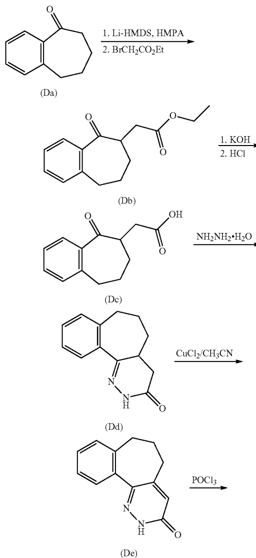
REACTION SCHEME 3
