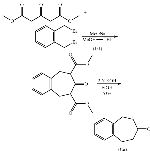
REACTION SCHEME 2B
