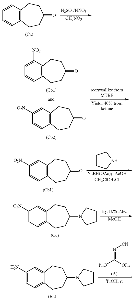
REACTION SCHEME 2
