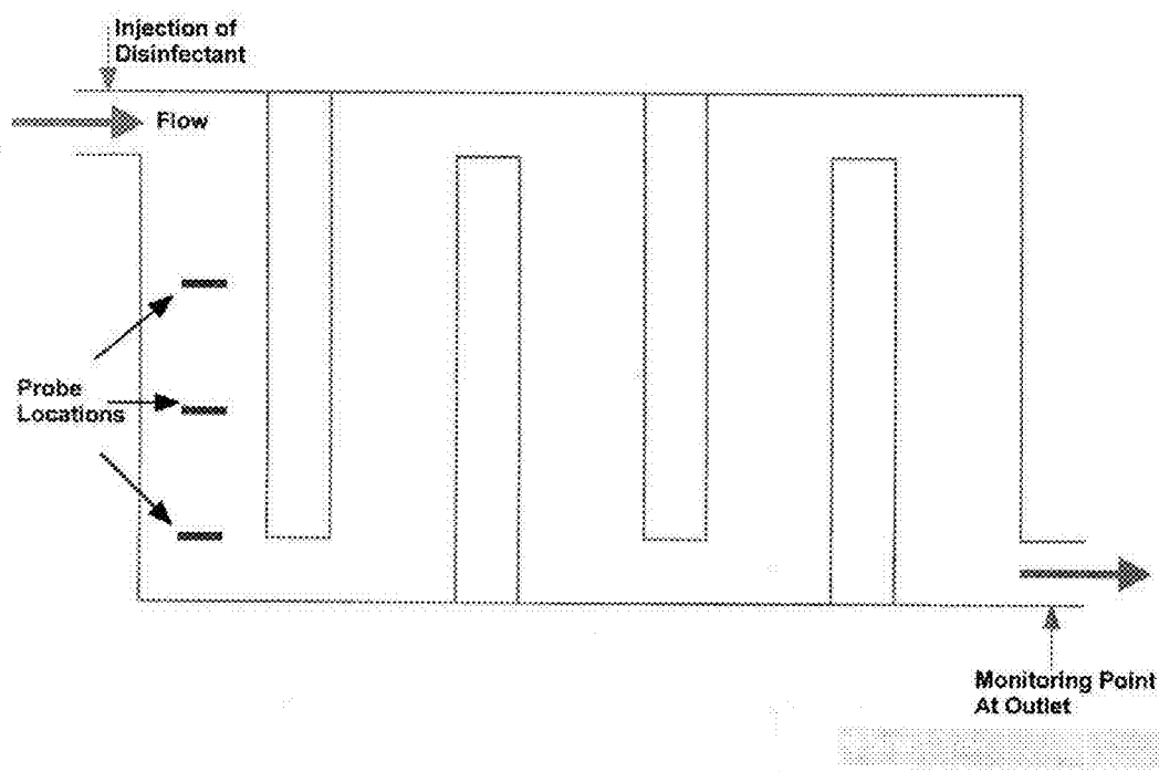
Figure 7. Disinfectant probe locations in a contact chamber.
