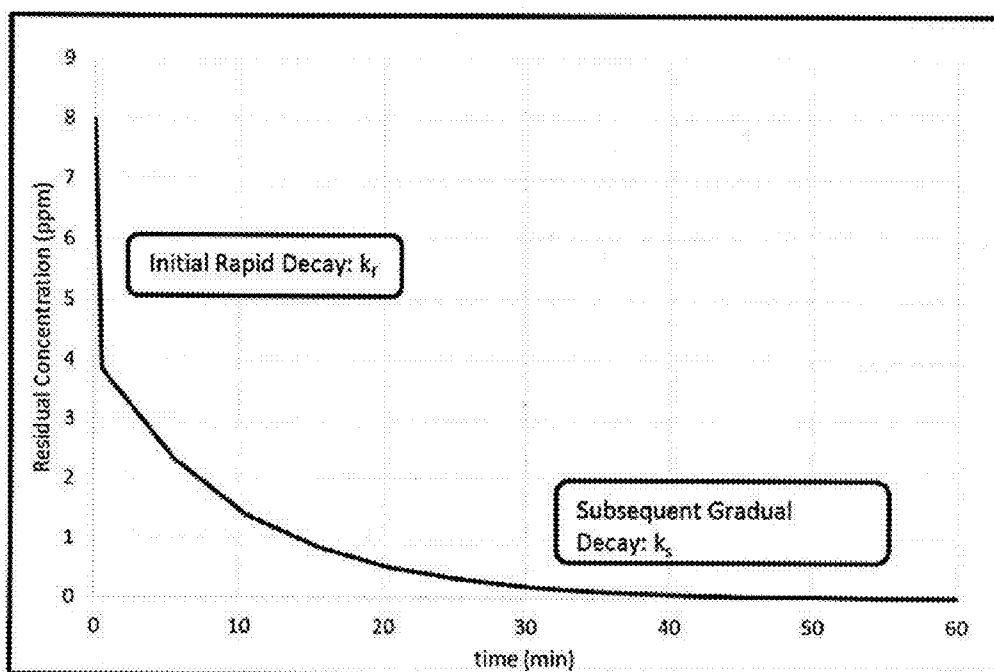
Figure 2. An example of PAA decay in a wastewater sample.
