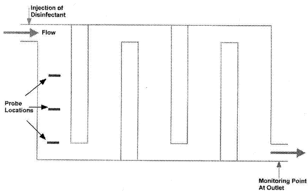
Figure 4. Disinfectant probe locations in a contact chamber.
