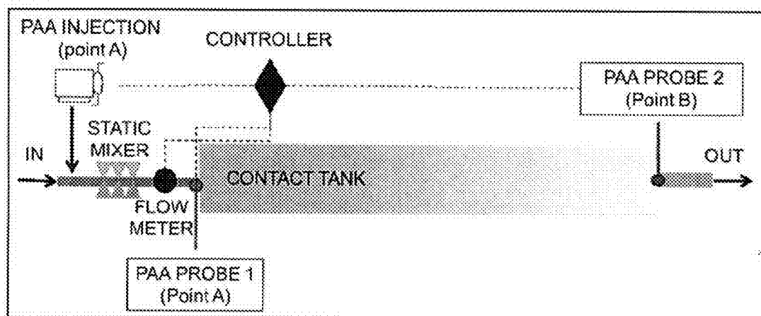
Figure 12. A schematic of the plant installation
