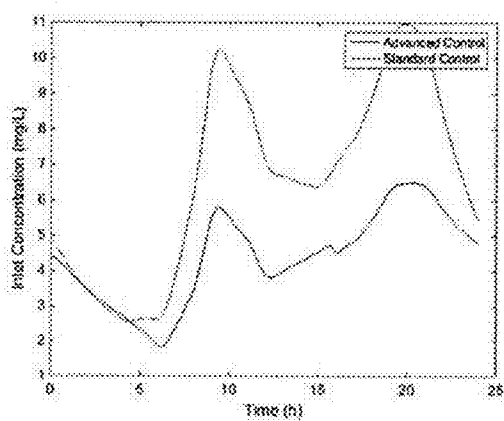
Figure 6. PAA Usage and Microbial Disinfection Performance for the Primary Wastewater Demand/Decay Parameters.
