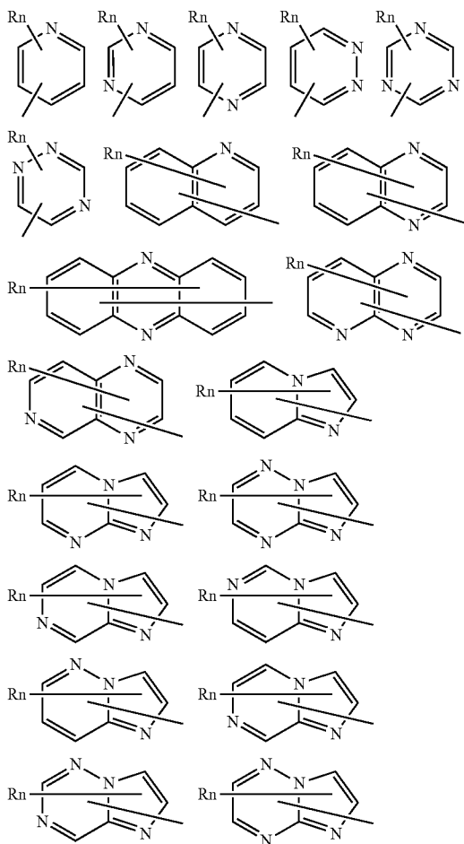
[Chem. 39]
