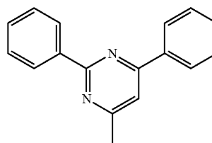
[Chem. 40]
