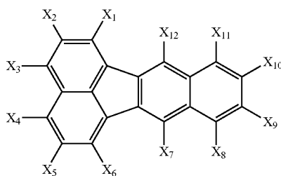
[Chem. 30]
