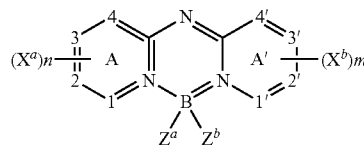
[Chem. 31]
