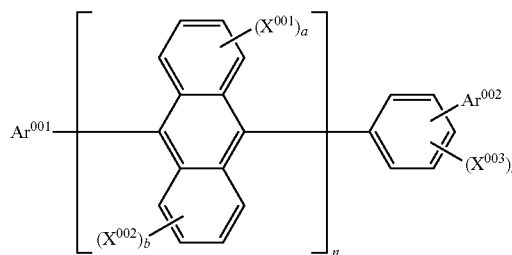
[Chem. 32]
