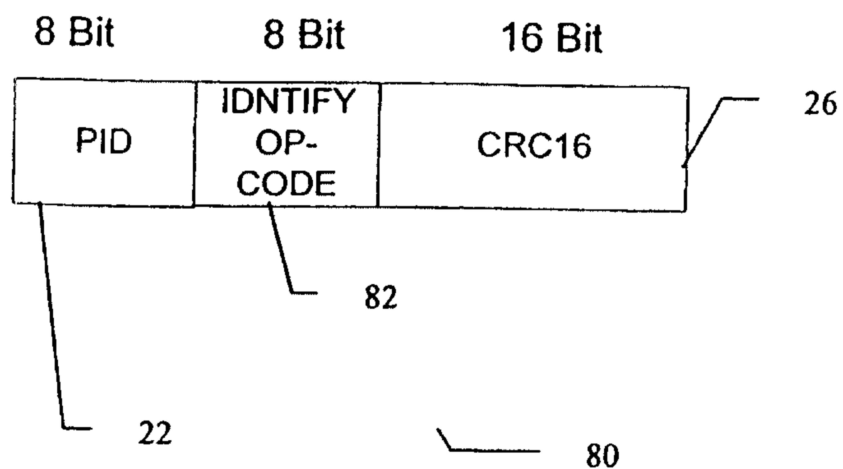
Fig 7 – Flash Identification Request Packet
