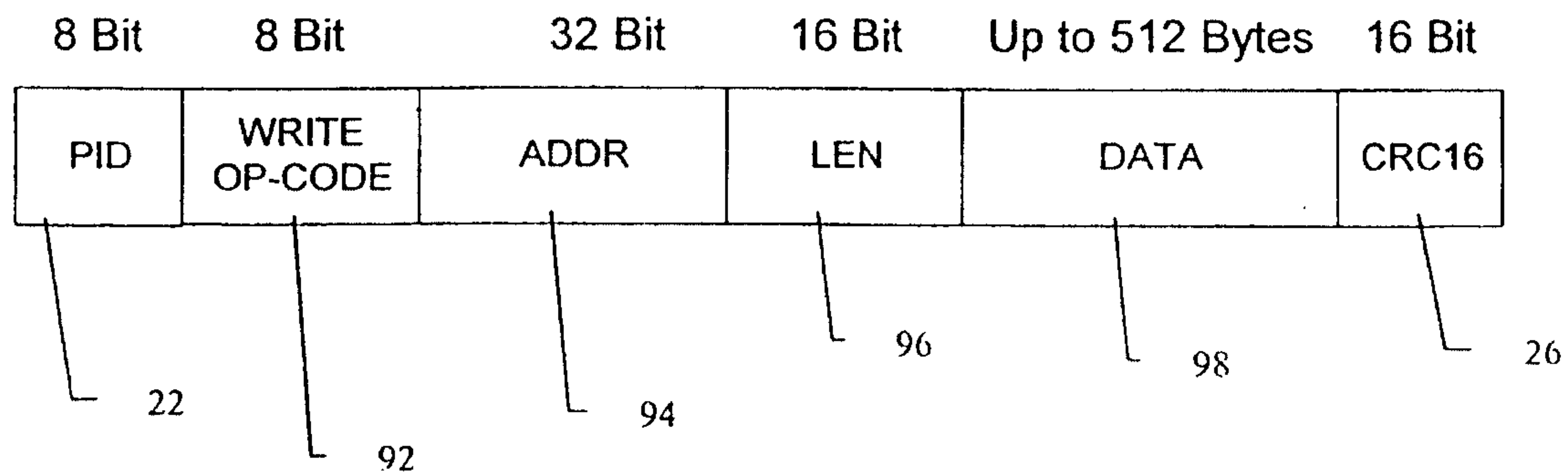
Fig 9 –Write Request Packet
