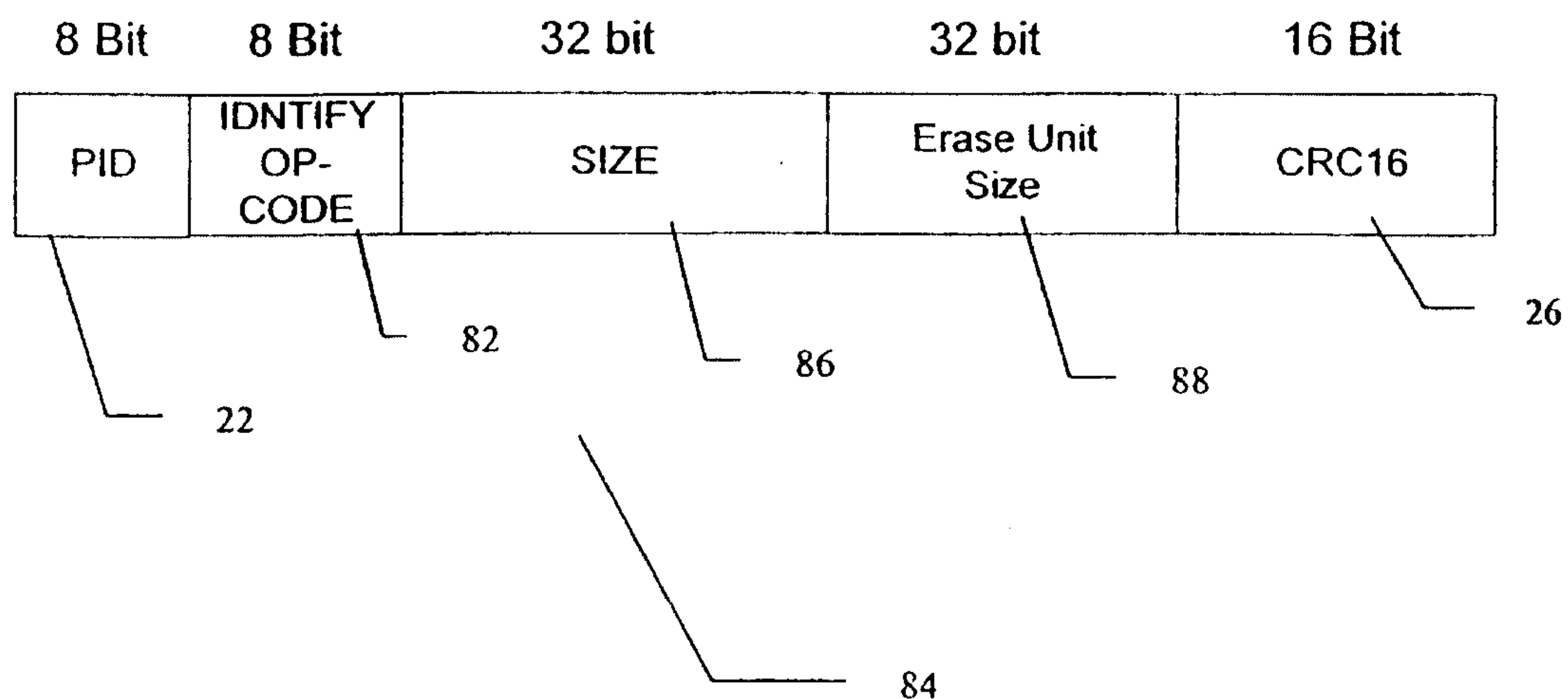
Fig 8 – Flash Identification Replay Packet
