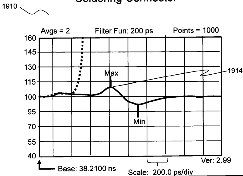
FIG. 19B Soldering Connector
