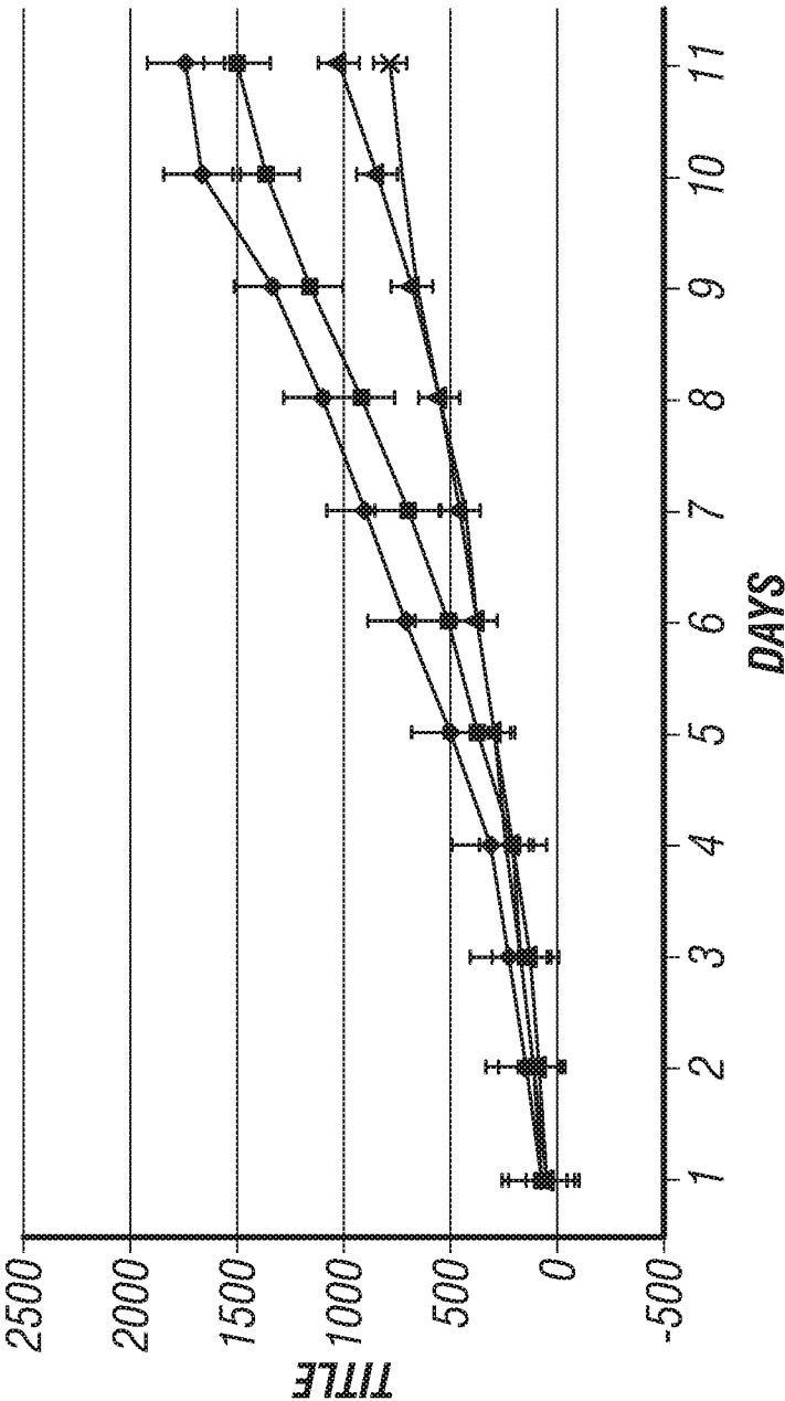
AD-RLX+AD-IL24+ANTI-PD-1 EFFICACY ◆-- PBS ■-- Anti-PD-1 ▲-- Ad-RLX+Ad-IL24 ✕-- Ad-RLX+Ad-IL24+Anti-PD-1
