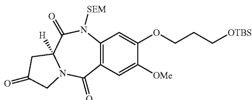
8-[3-(tert-Butyl-dimethyl-silyloxy)-propoxy]-7-methoxy-10-(2-trimethylsilylanyl-ethoxymethyl)-1,11a-dihydro-1 OH-benzo[e]pyrrolo[1,2-a][1,4]diazepine-2,5,11-trione (11)
