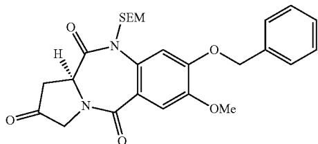
8-Benzyloxy-7-methoxy-10-(2-trimethylsilyl-ethoxymethyl)-1,11a-dihydro-10H-benzo[e]pyrrolo[1,2-a][1,4]diazepine-2,5,11-trione (13)
