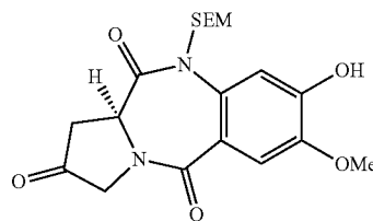
8-Hydroxy-7-methoxy-10-(2-trimethylsilyl-ethoxymethyl)-1,11a-dihydro-10H-benzo[e]pyrrolo[1,2-a][1,4]diazepine-2,5,11-trione (12)
