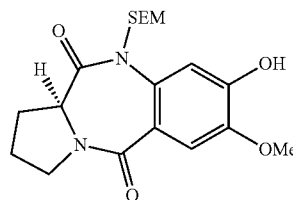
8-Hydroxy-7-methoxy-10-(2-trimethylsilylanyl-ethoxymethyl)-1,2,3,11a-tetrahydro-10H-benzo[e]pyrrolo[1,2-a][1,4]diazepine-5,11-dione (3)
