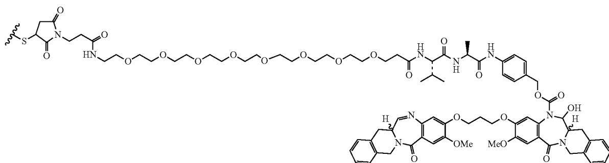
Formula IV
