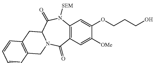
2-(3-Hydroxy-propoxy)-3-methoxy-13-(2-trimethylsilylanyl-ethoxymethyl)-11,11a-dihydro-6H,13H-5a,13-diaza-benzo[4,5]cyclohepta[1,2-b]naphthalenene-5,12-dione (4)
