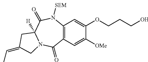
2-Ethylidene-8-(3-hydroxy-propoxy)-7-methoxy-10-(2-trimethylsilylanyl-ethoxymethyl)-1,2,3,11a-tetrahydro-10H-benzo[e]pyrrolo[1,2-a][1,4]diazepine-5,11-dione (9)
