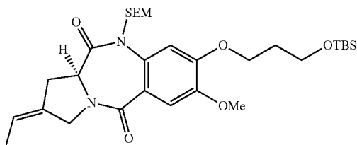
8-[3-(tert-Butyl-dimethyl-silyloxy)-propoxy]-2-ethylidene-7-methoxy-10-(2-trimethylsilylanyl-ethoxymethyl)-1,2,3,11a-tetrahydro-10 OH-benzo[e]pyrrolo[1,2-a][1,4]diazepine-5,11-dione (10)
