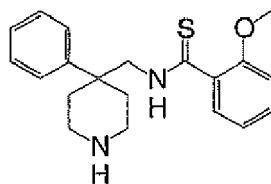
2-Methoxy-N-(4-phenyl-piperidin-4-ylmethyl)-thiobenzamide
