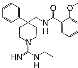
N-[1-(N-Ethylcarbamimidoyl)-4-phenyl-piperidin-4-ylmethyl]-2-methoxy-benzamide
