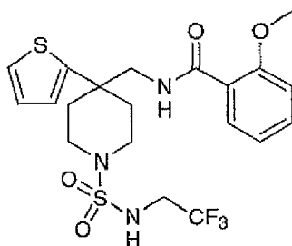
2-Methoxy-N-[4-thiophen-2-yl-1-(2,2,2-trifluoro-ethylsulfamoyl)-piperidin-4-ylmethyl]-benzamide
