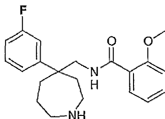
N-[4-(3-Fluoro-phenyl)-azepan-4-ylmethyl]-2-methoxy-benzamide
