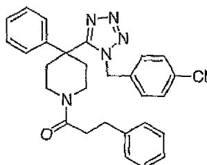
1-[4-[1-(4-Chloro-benzyl)-1H-tetrazol-5-yl]-4-phenyl-piperidin-1-yl]-3-phenyl-propan-1-one
