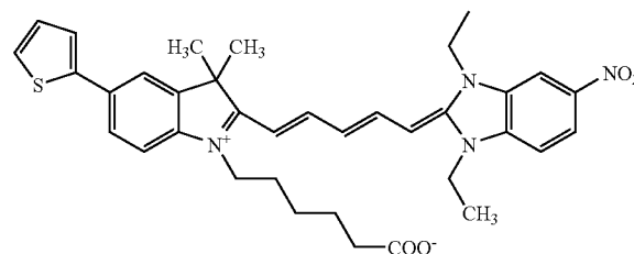
Compound 19
