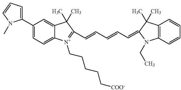
Compound 22
