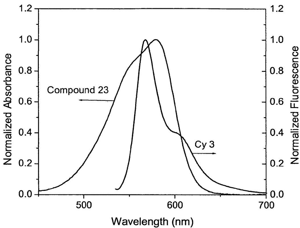
FIG. 9. Spectral overlap of compound 23 with Cy3
