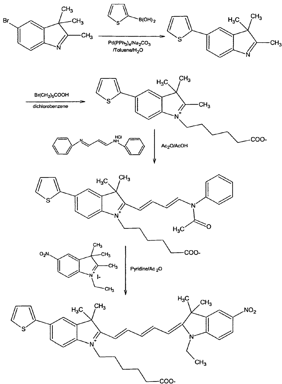
FIG. 7. Synthesis of a cyanine that has a LQM at Ring A or Ring B
