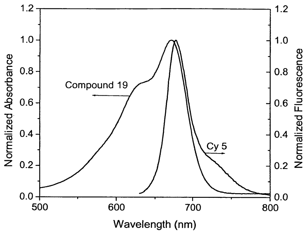
FIG. 10. Spectral overlap of compound 19 with Cy5.
