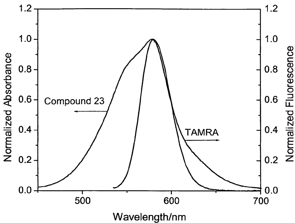
FIG. 8. Spectral overlap of compound 23 with 5-TAMRA
