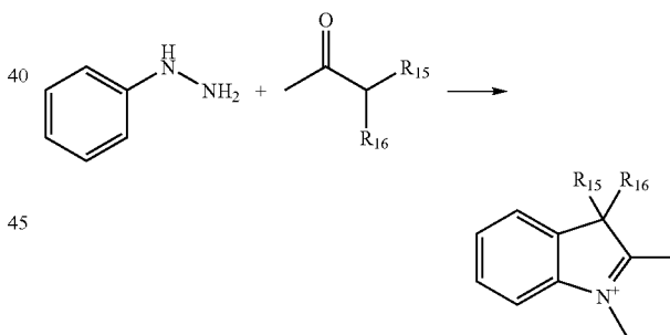
Scheme 1. Typical synthesis of indolium intermediates
