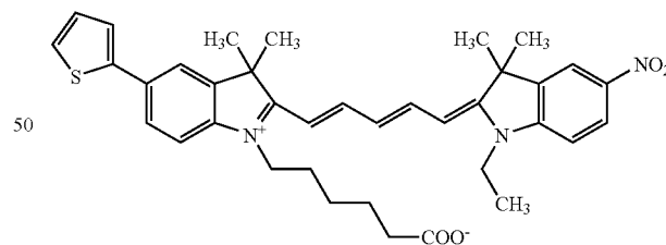
Compound 16 35
