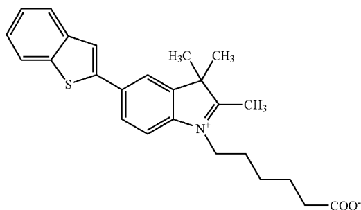
Compound 13 40
