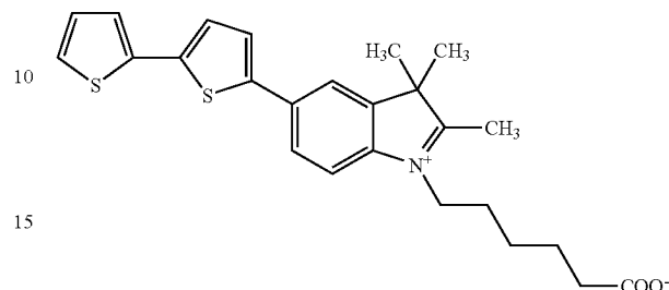
Compound 14 10
