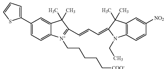
Compound 23
