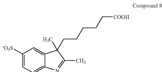
Compound 8
