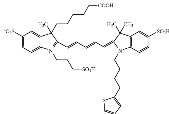
Compound 10
