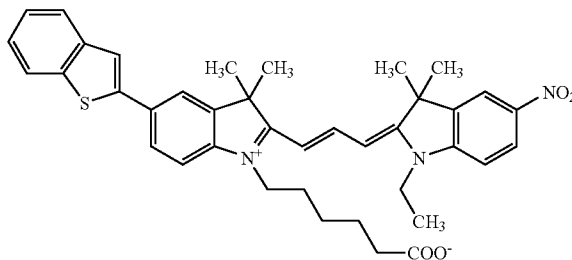
Compound 24
