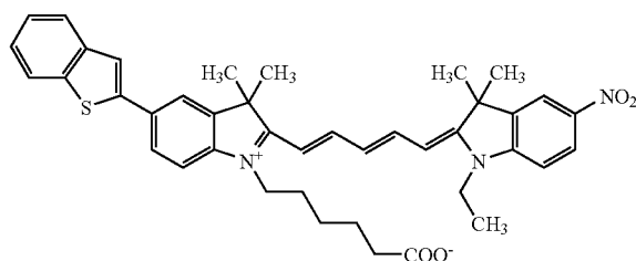
Compound 18 50
