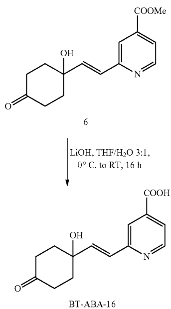
Scheme 17-3
