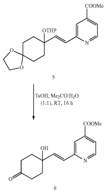
Scheme 17-2
