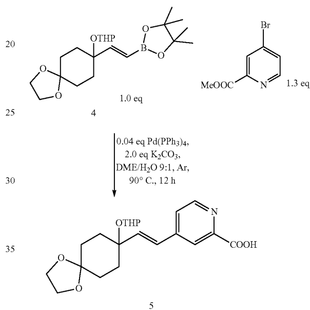
Scheme 18-1
