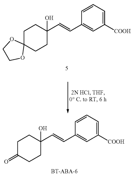
Scheme 15-3
