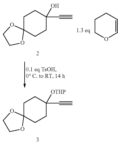
Scheme 16-1
