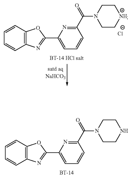
Scheme 4-3
