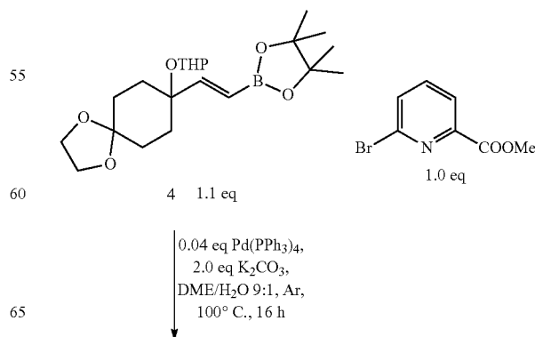
Scheme 16-4
