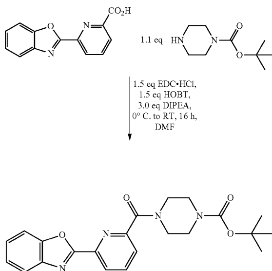
Scheme 4-1
