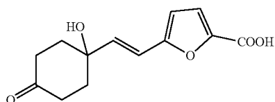
Scheme 13-1
