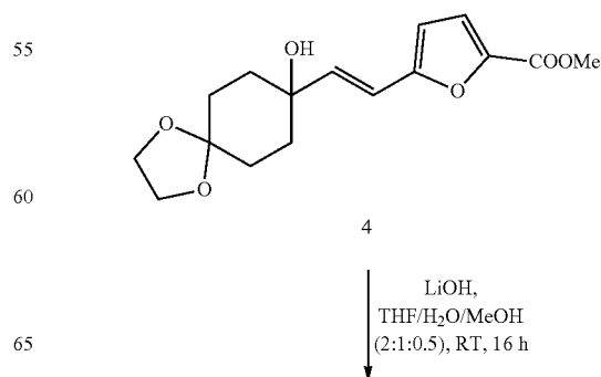
Scheme 14-2
