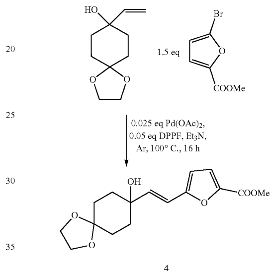
Scheme 14-1
