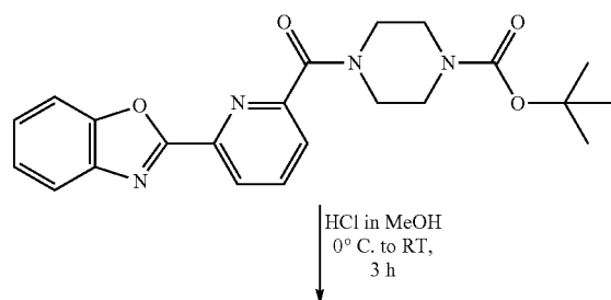
Scheme 4-2
