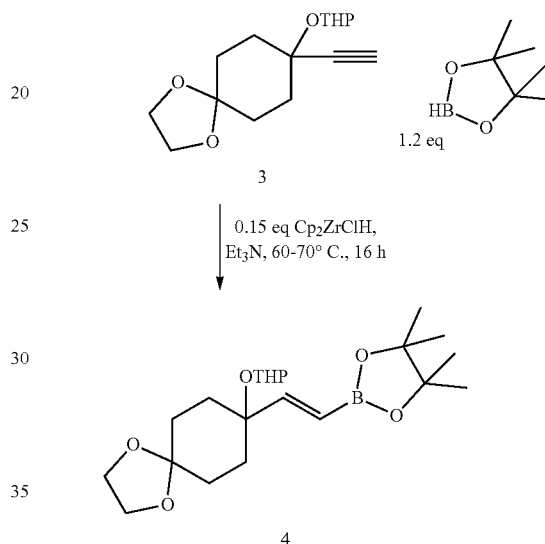
Scheme 16-2
