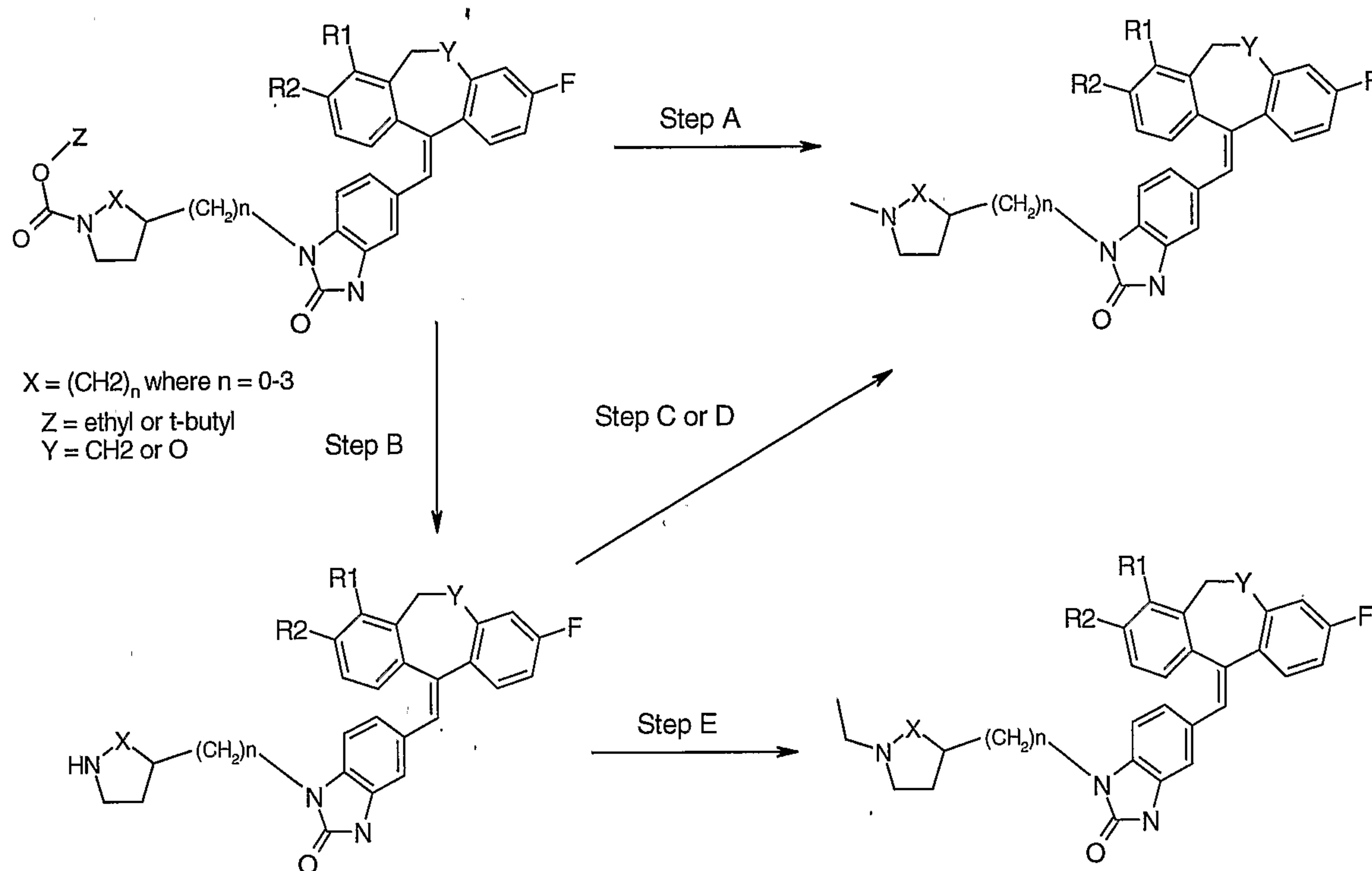
Scheme IV
