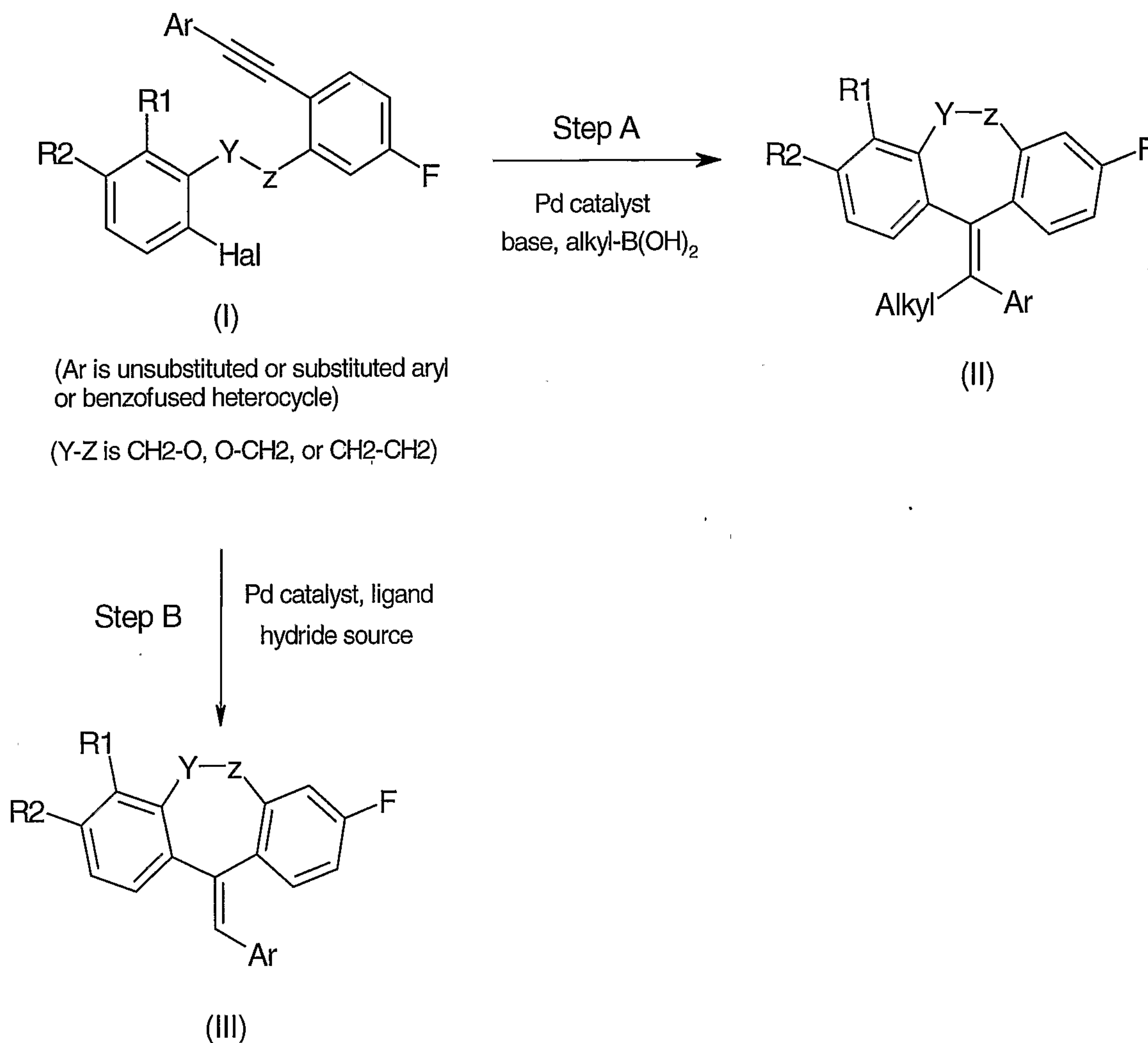
Scheme VII (a)
