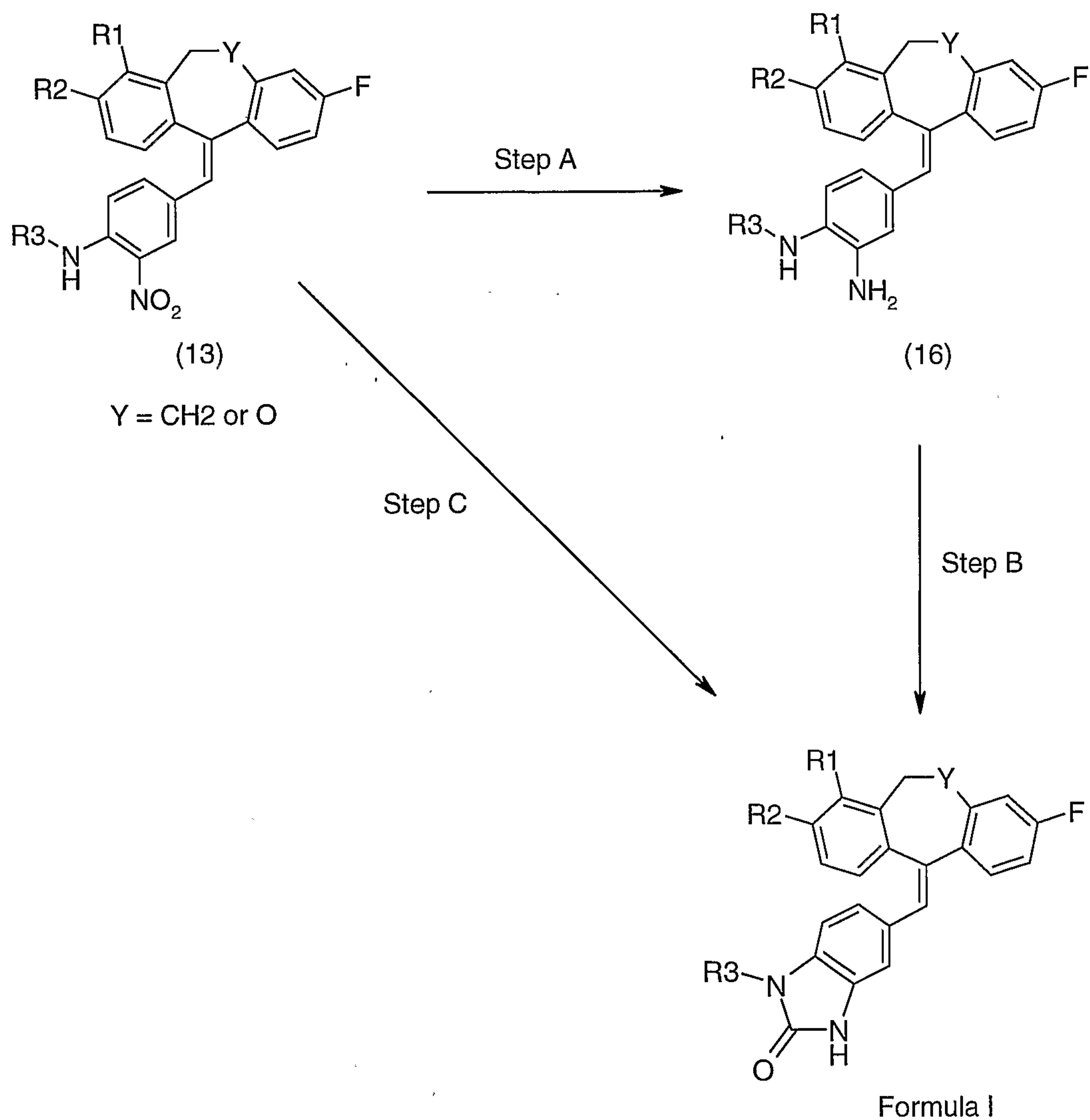
Scheme V(b)
