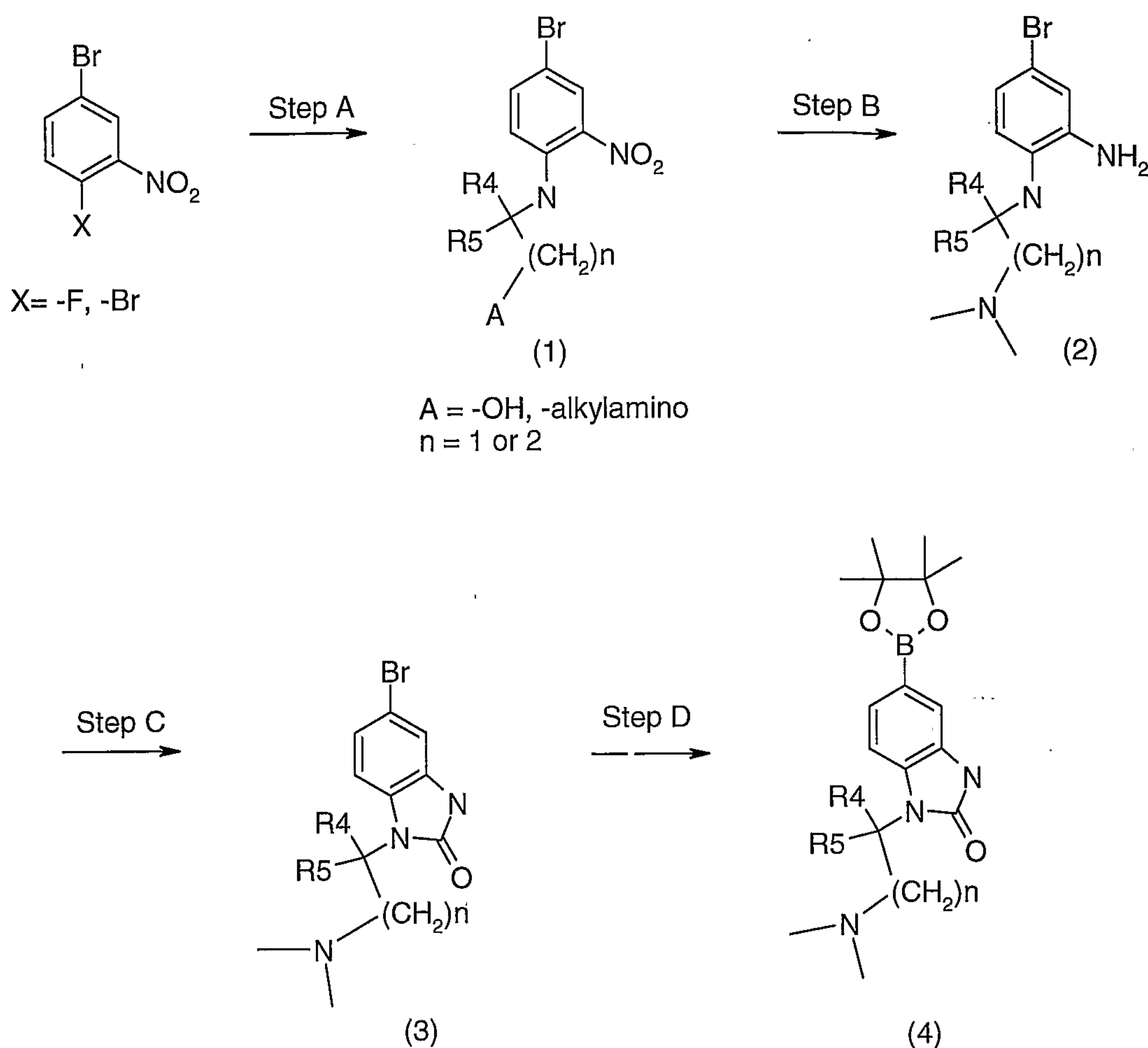
Scheme I
