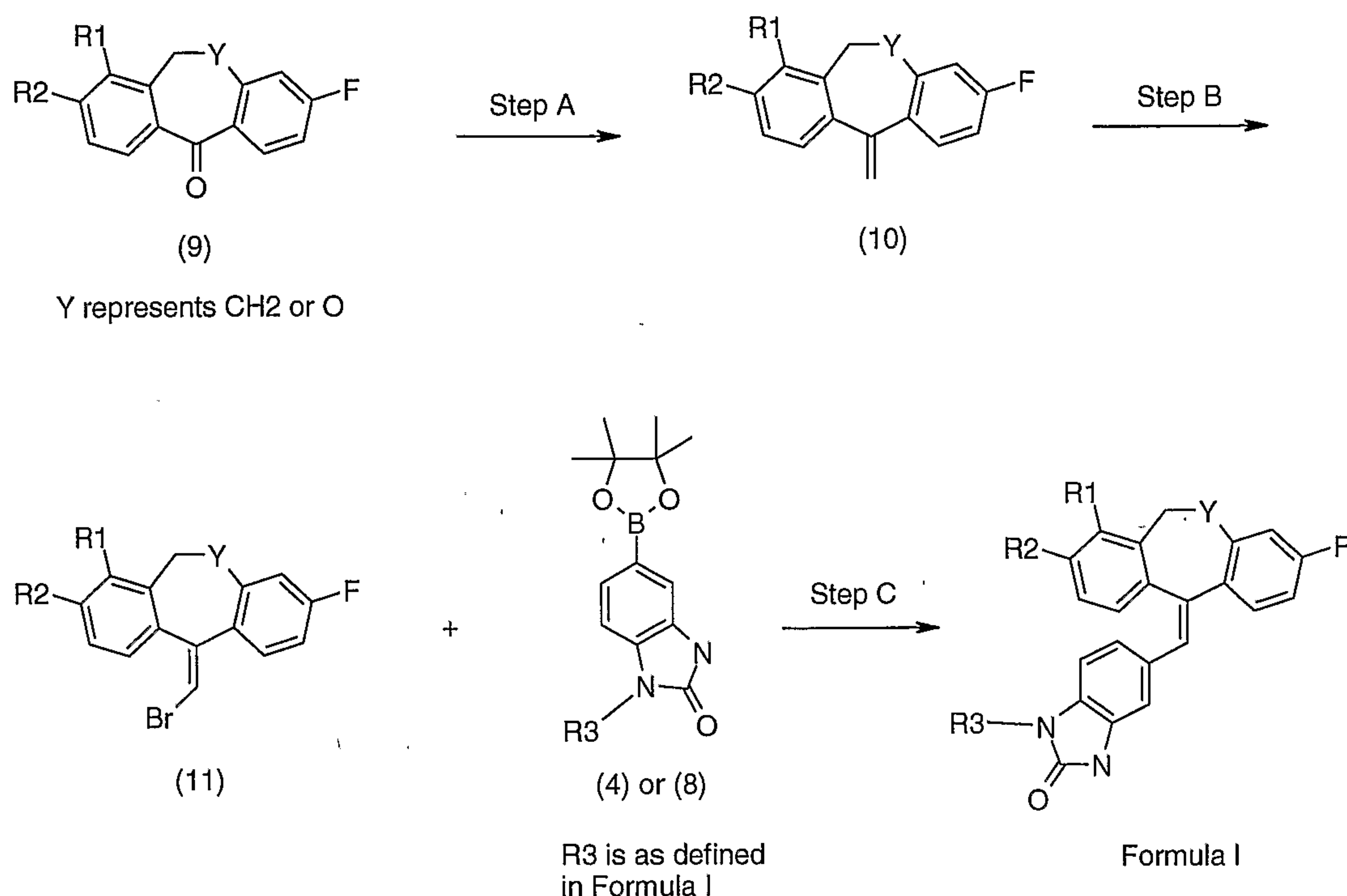
Scheme III
