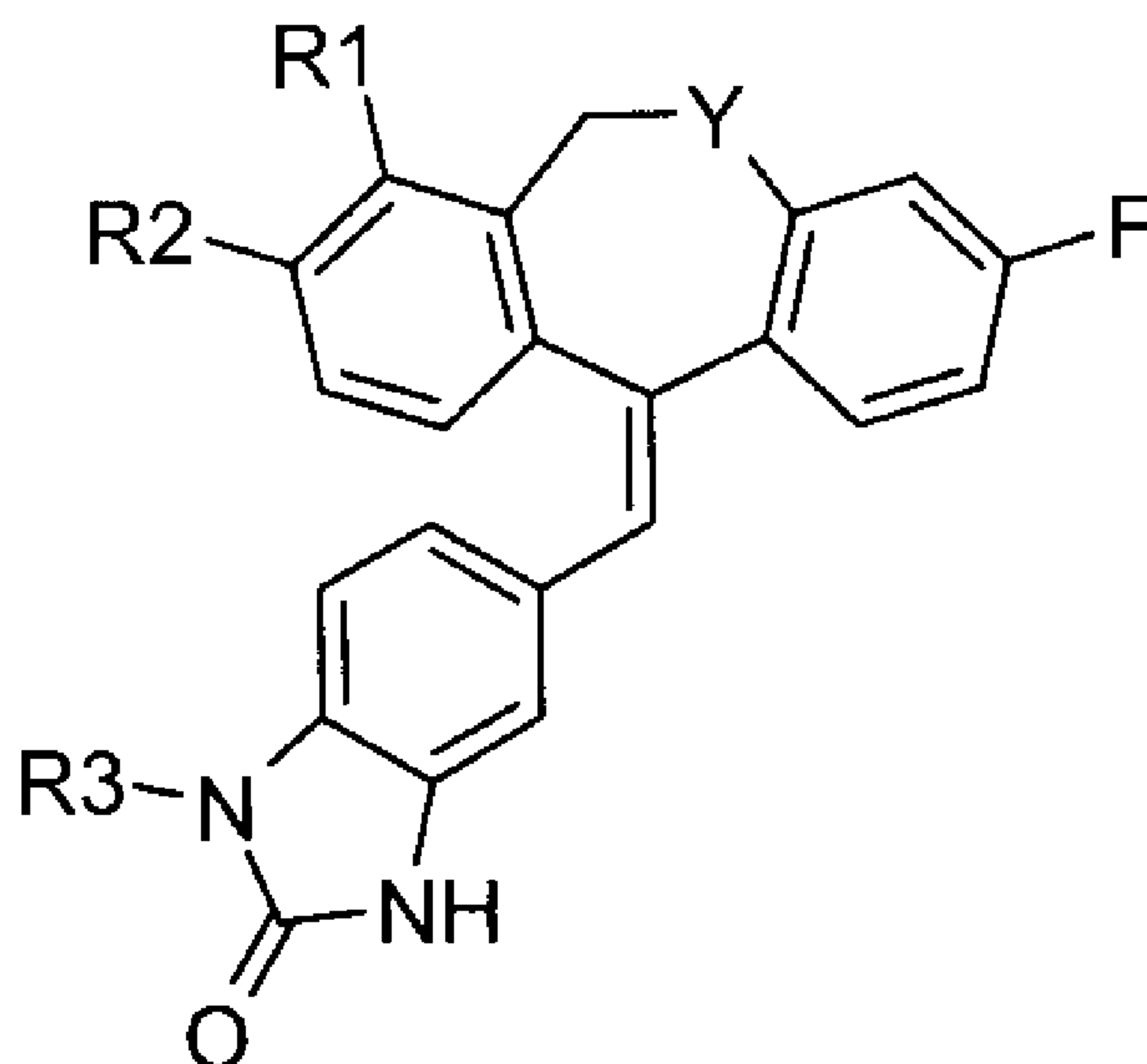
Formula I
