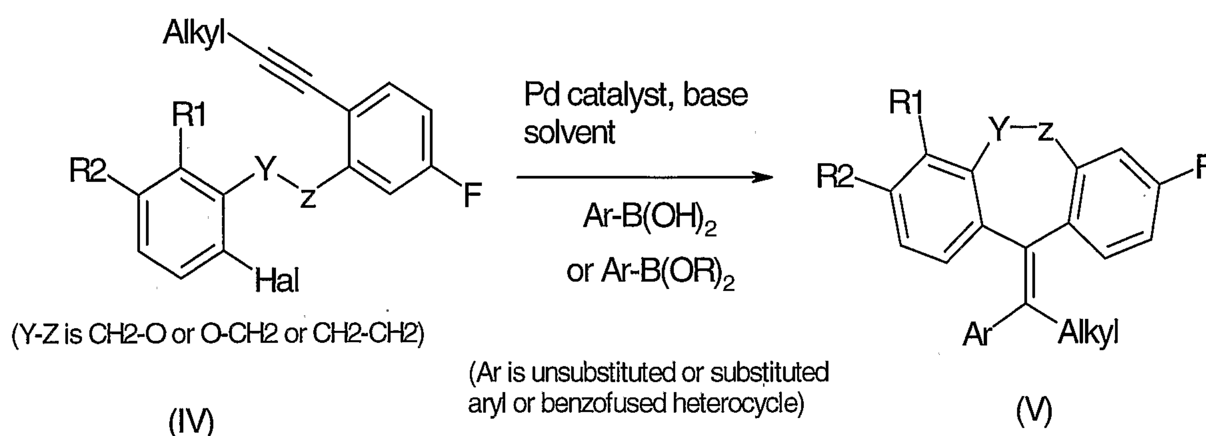
Scheme VII(b)
