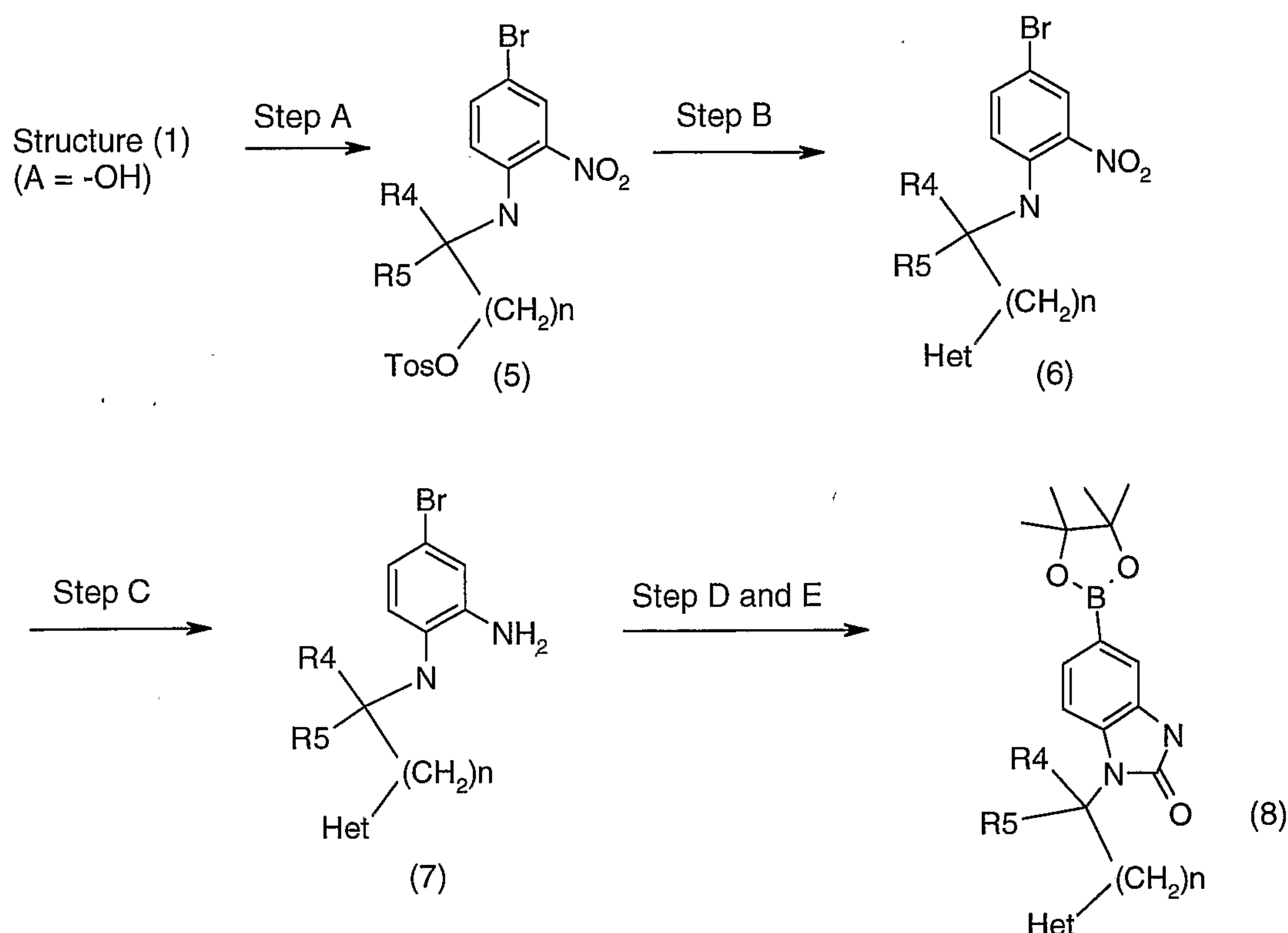
Scheme II
