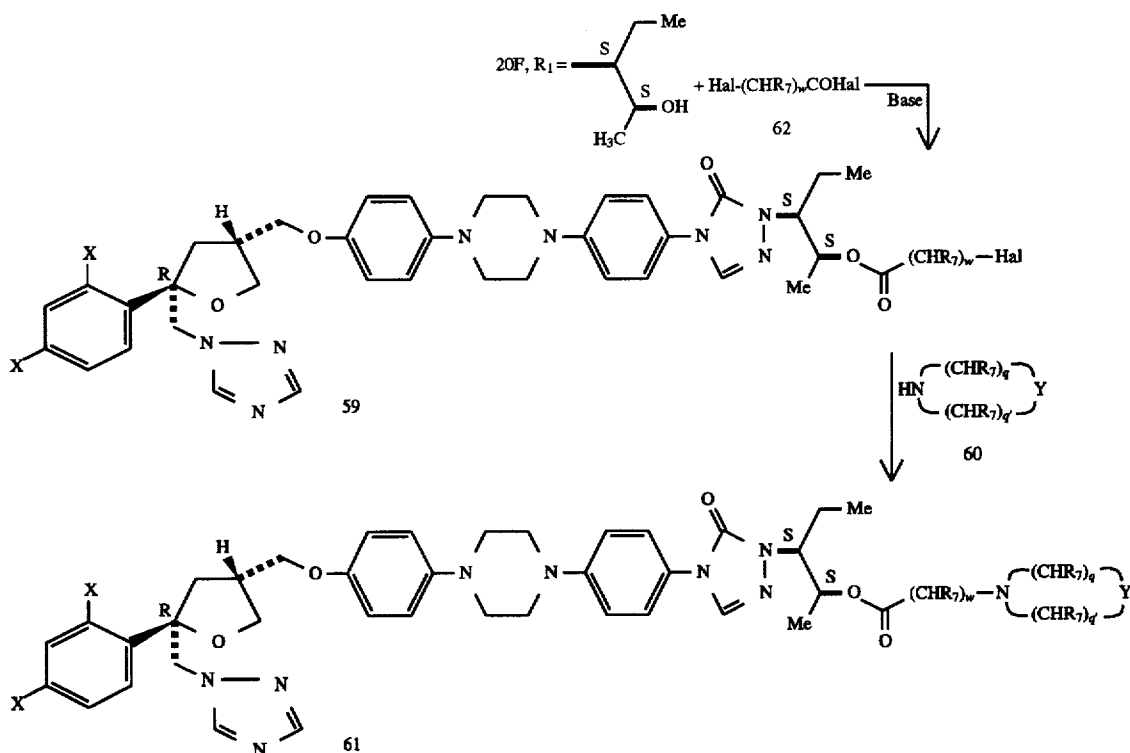
Scheme IX Preparation of Heterocyclic Esters
