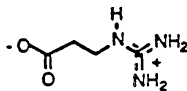
\beta -guanidino-propionic acid (VI)
