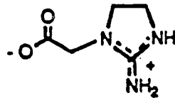
1-carboxymethyl-2-iminoimidazolidine
