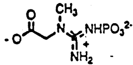
N-phosphoryl creatine
