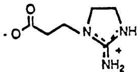
1-carboxyethyl-2-iminoimidazolidine (IV)
