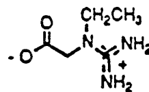
N-ethyl-N-amidino-glycine (V)
