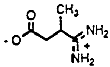
3-amidinobutyric acid (III) "Carbocreatine"
