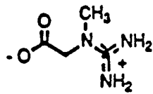
Creatine
