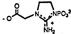
3-Phosphoryl-1-carboxymethyl-2-iminoimidazolidine
