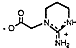
1-carboxymethyl-2-iminohexa-hydropyrimidine (II)
