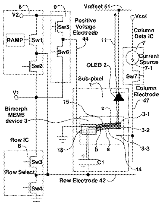
BIMORPH MEMS DEVICE POSITIONED LIGHT EMISSION
