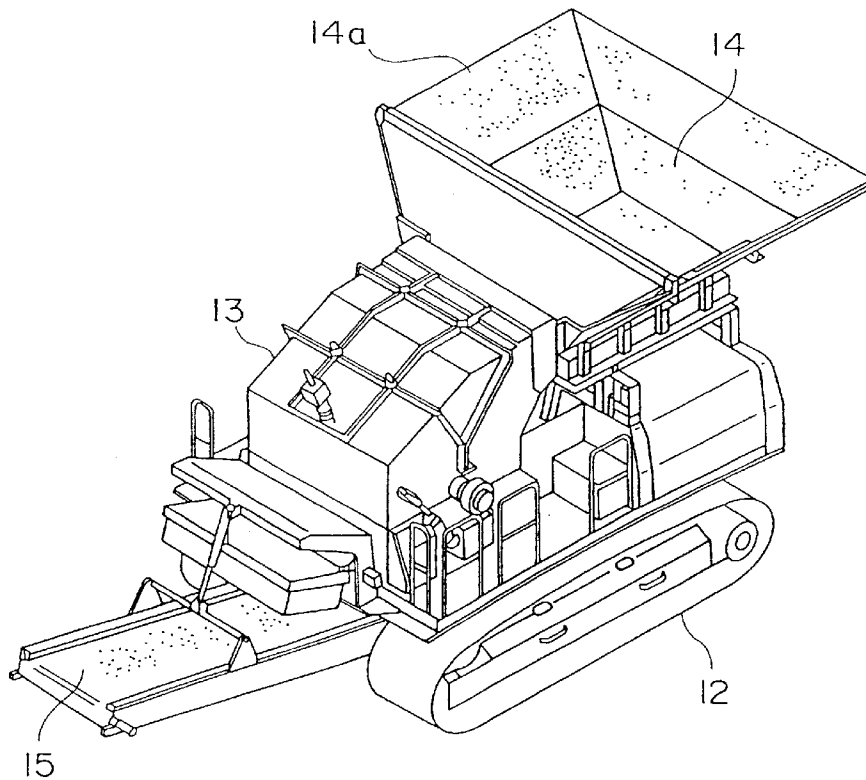
FIG. 9 CONVENTIONAL ART
