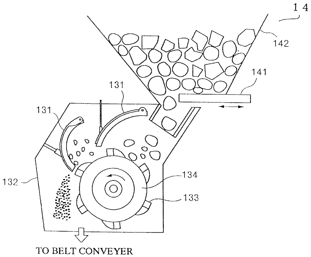
FIG. 10 CONVENTIONAL ART
