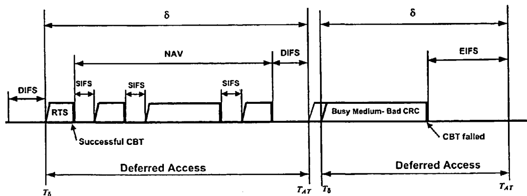
Figure 8— Fast Adaptation timing - Observed successful RTS and observed transmission failure
