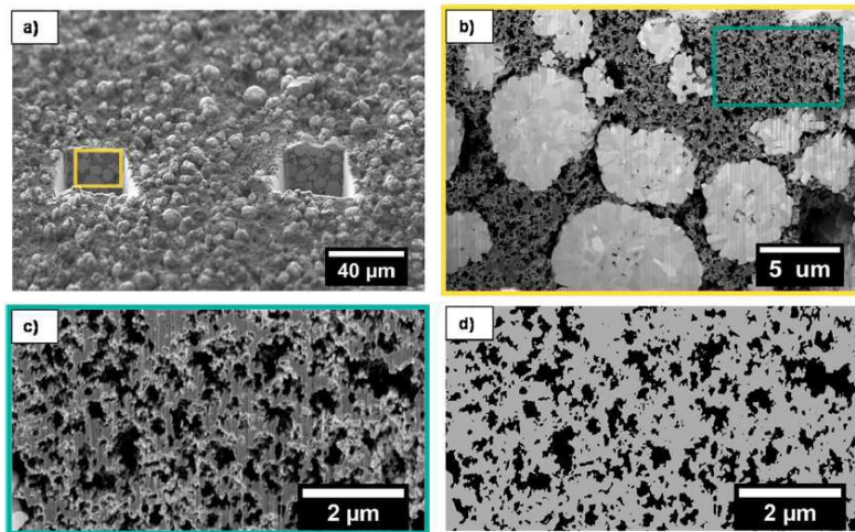
Figure 2. (a) SEM micrograph taken at 500 \times depicting two of the trenches milled into the NMC electrode. The yellow box depicts the area of focus of the serial sectioning. (b) SEM micrograph taken at 4000 \times depicting the electrode with the green box outlining the CBD slice used successively. (c) Closeup of the SEM micrograph in panel b. (d) Threshold segmentation of the image in panel c.
