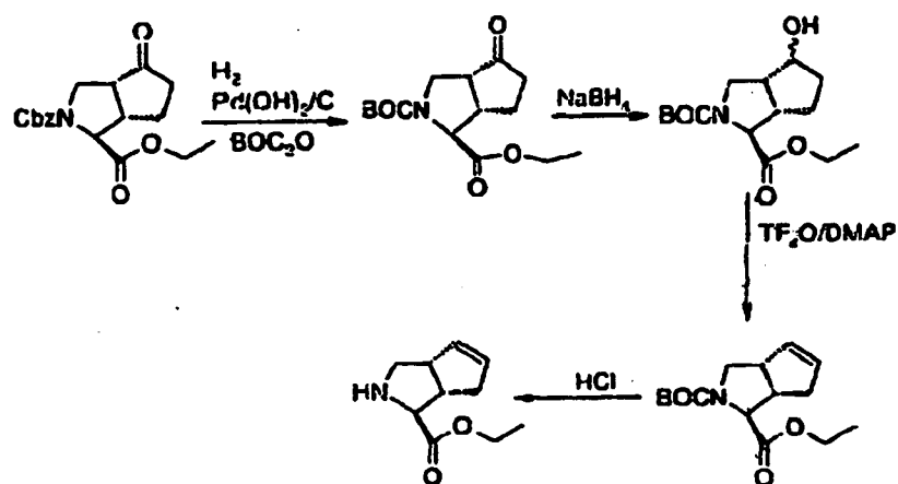
SCHEME 7
