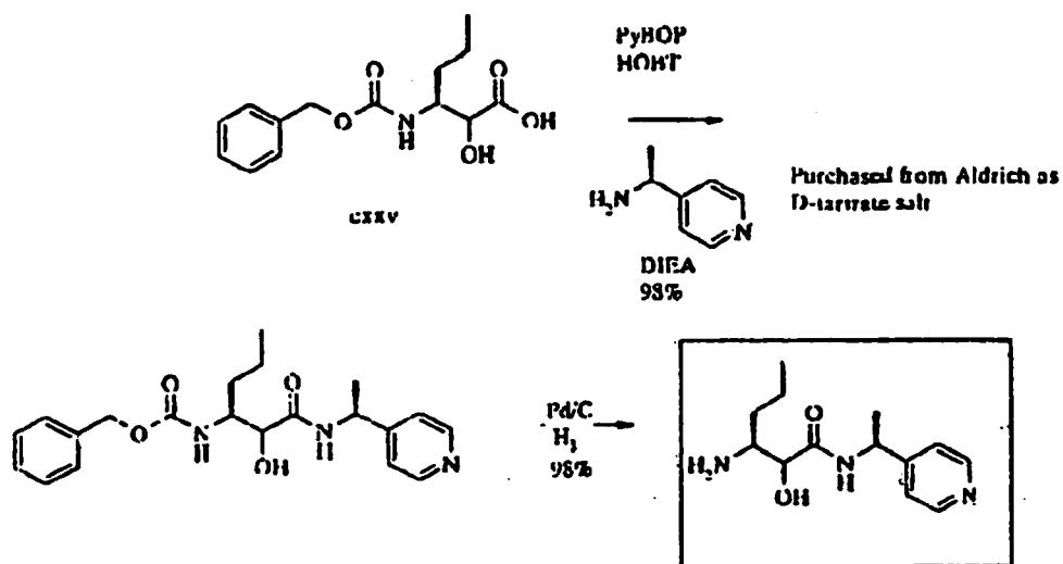
SCHEME 10
