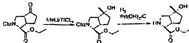
SCHEME 5
