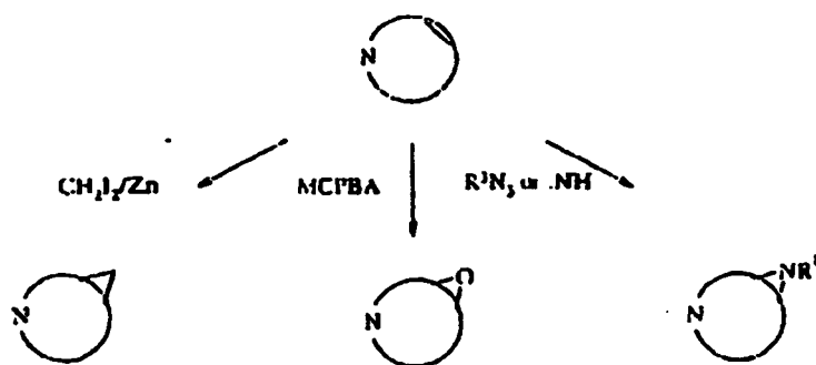
SCHEME 8
