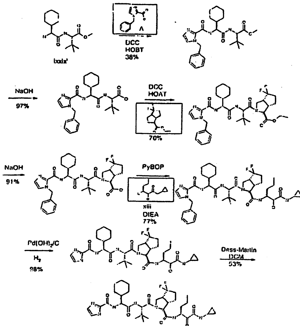
Scheme 11
