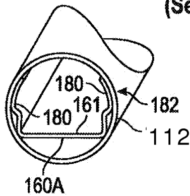
FIG. 6C (Section C-C)
