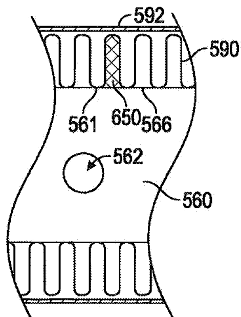
FIG. 12C (Section H-H)
