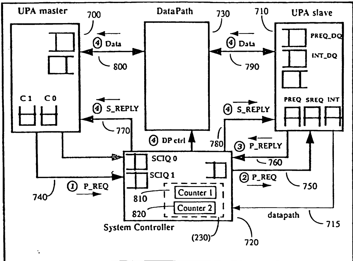
Slave Read Flow Control
