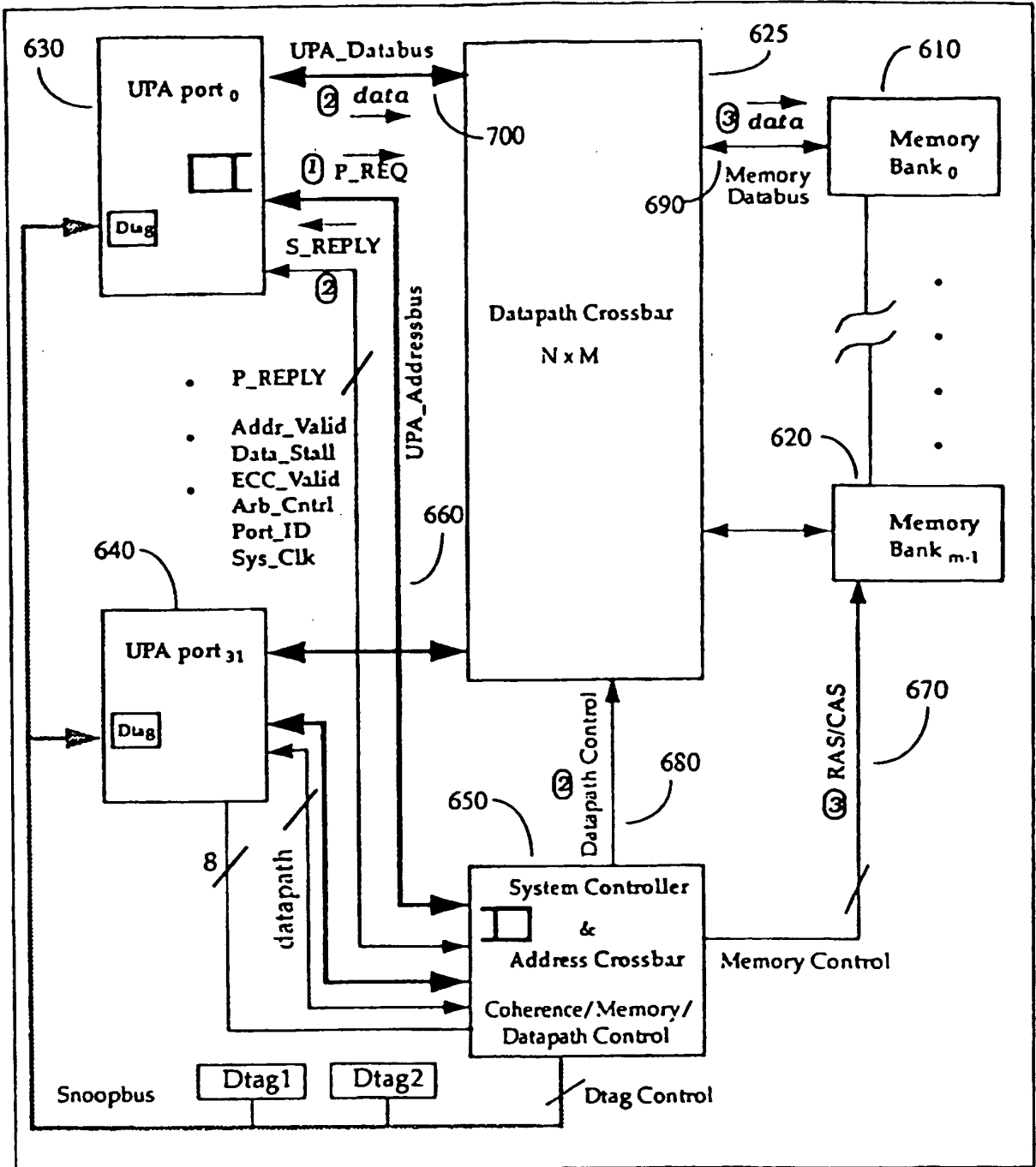
Memory Write Flow Control
