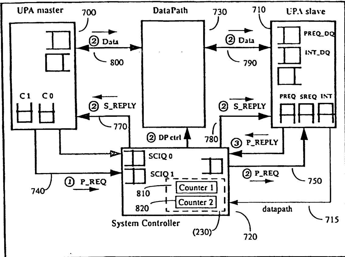
Slave Write Flow Control
