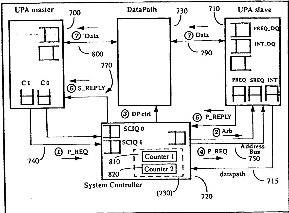
Slave Read Flow Control: Circuit-Switched
