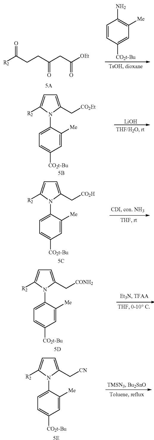
Scheme 5: A general scheme for preparing GSNOR inhibitors with structure 5H
