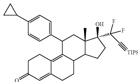
17α-[1,1-difluoro-3-[tris(1-methylethyl)silyl]-2-propyn-1-yl]-17β-hydroxy-11β-[4-p-(cyclopropyl)phenyl]estra-4,9-dien-3-one. (6a)
