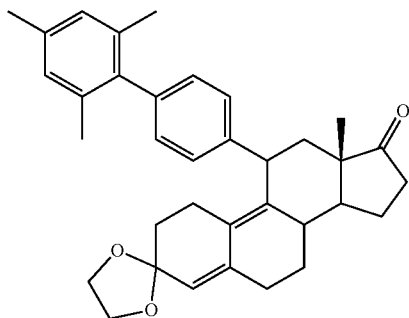
3,3-Ethylendioxy-11β-[4-p-(2,4,6-trimethylphenyl)phenyl]estra-4,9-dien-17-one (4k)
