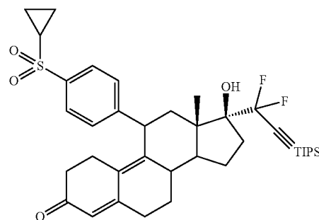
17α-[1,1-difluoro-3-[tris(1-methylethyl)silyl]-2-propyn-1-yl]-17β-hydroxy-11β-[4-p-(cyclopropylthio)sulfonyl]phenyl]estra-4,9-dien-3-one (61)
