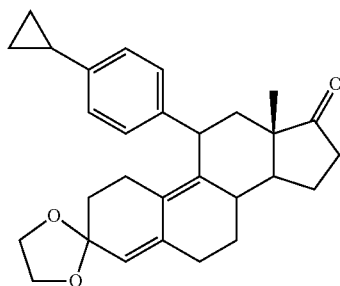
3,3-Ethylendioxy-11β-[4-p-(cyclopropyl)phenyl]estra-4,9-dien-17-one (4a)
