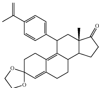
3,3-Ethylendioxy-11β-[4-p-(1-methylethenyl)phenyl]estra-4,9-dien-17-one (4 g)
