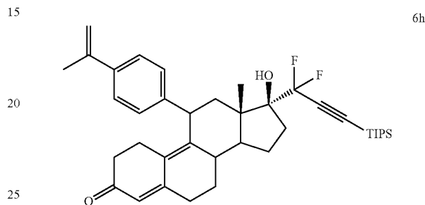
17α-[1,1-difluoro-3-[tris(1-methylethyl)silyl]-2-propyn-1-yl]-17β-hydroxy-11β-[4-p-(1-methylethenyl)phenyl]estra-4,9-dien-3-one (6h)
