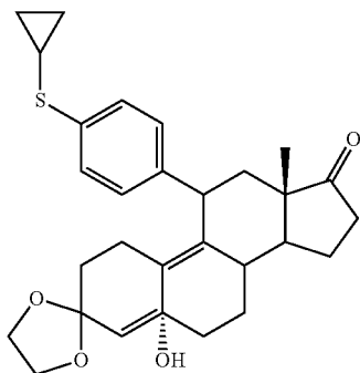
3,3-Ethylendioxy-5α-hydroxy-11β-[4-p-(cyclopropylthio)phenyl]estra-9-en-17-one (31)
