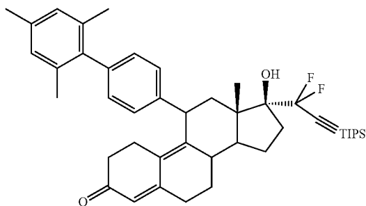
17α-[1,1-difluoro-3-[tris(1-methylethyl)silyl]-2-propyn-1-yl]-17β-hydroxy-11β-[4-p-(2,4,6-trimethylphenyl)phenyl]estra-4,9-dien-3-one (6k)
