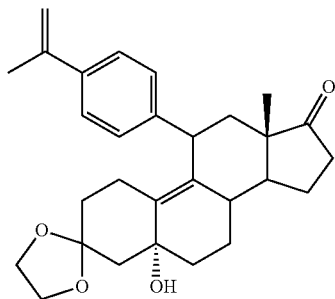
3,3-Ethylendioxy-5α-hydroxy-11β-[4-p-(1-methylethenyl)phenyl]estra-9-en-17-one (3 g)
