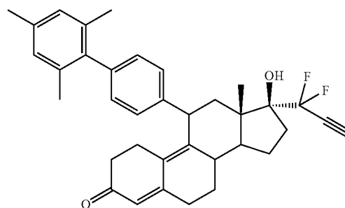
17α-(1,1-difluoro-2-propyn-1-yl)-17β-hydroxy-11β-[4-p-(2,4,6-trimethylphenyl)phenyl]estra-4,9-dien-3-one (EC359)
