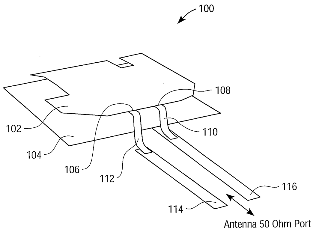
FIG. 1 (Prior Technology)
