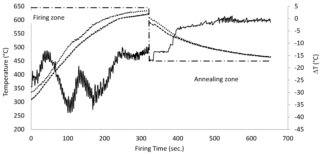
FIG. 3 ····· Comparative Example C - - - - Example 1 - · - · - Furnace Setup — ΔT (°C)
