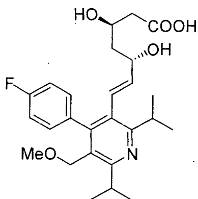
Cerivastatin
