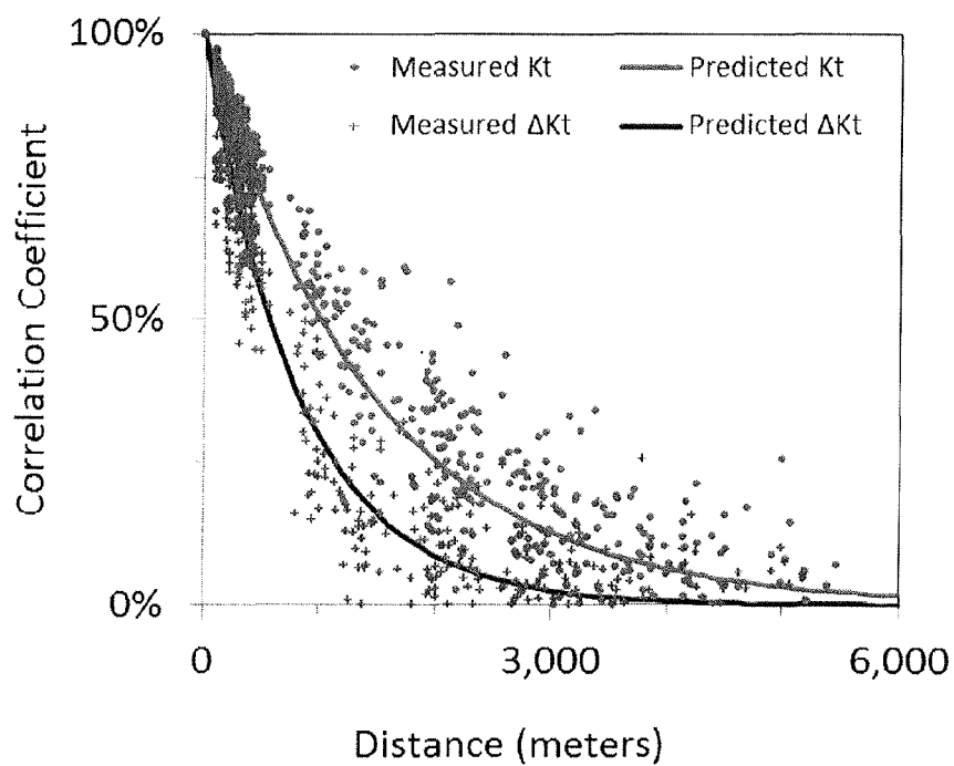
Correlation vs. Distance ( \Delta t=300 )
