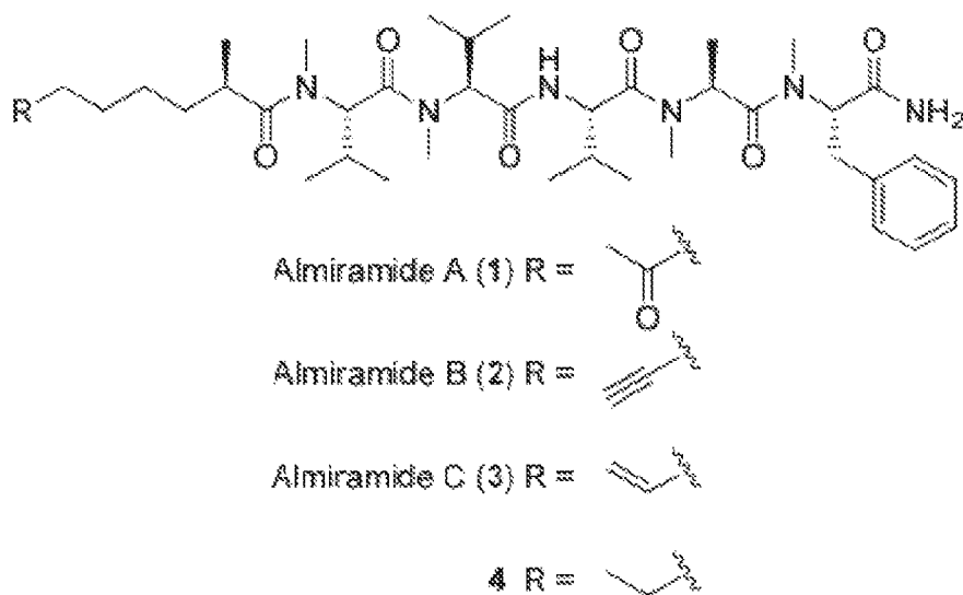
FIG. 1a: Almiramides A, B and C
