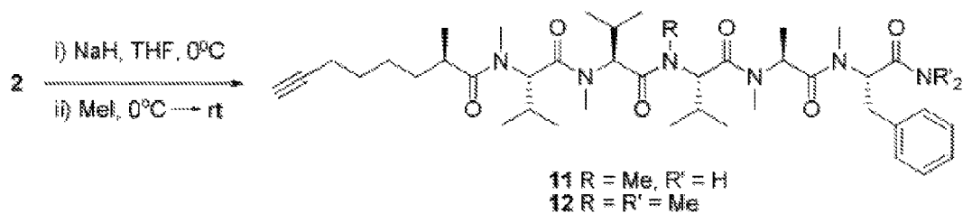
FIG.6 Formation of semi-synthetic derivatives 11 and 12.
