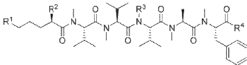
FIG. 4. Generic structure of Almiraide.
