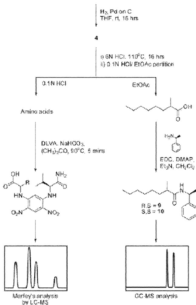
FIG.5 Configurational analysis strategy for 2 and 3.
