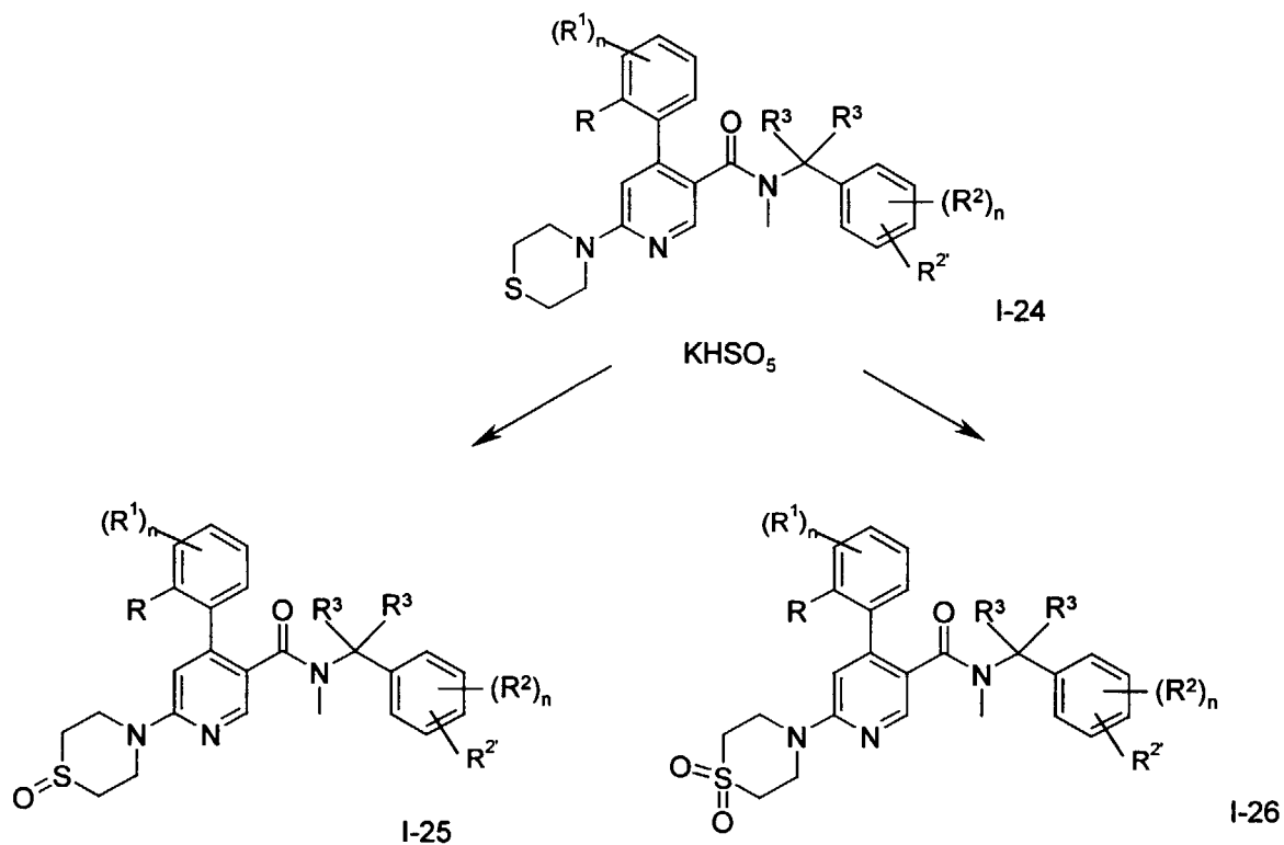
Scheme 8
