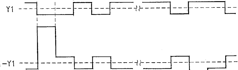
FIG.-43D (PRIOR ART)
