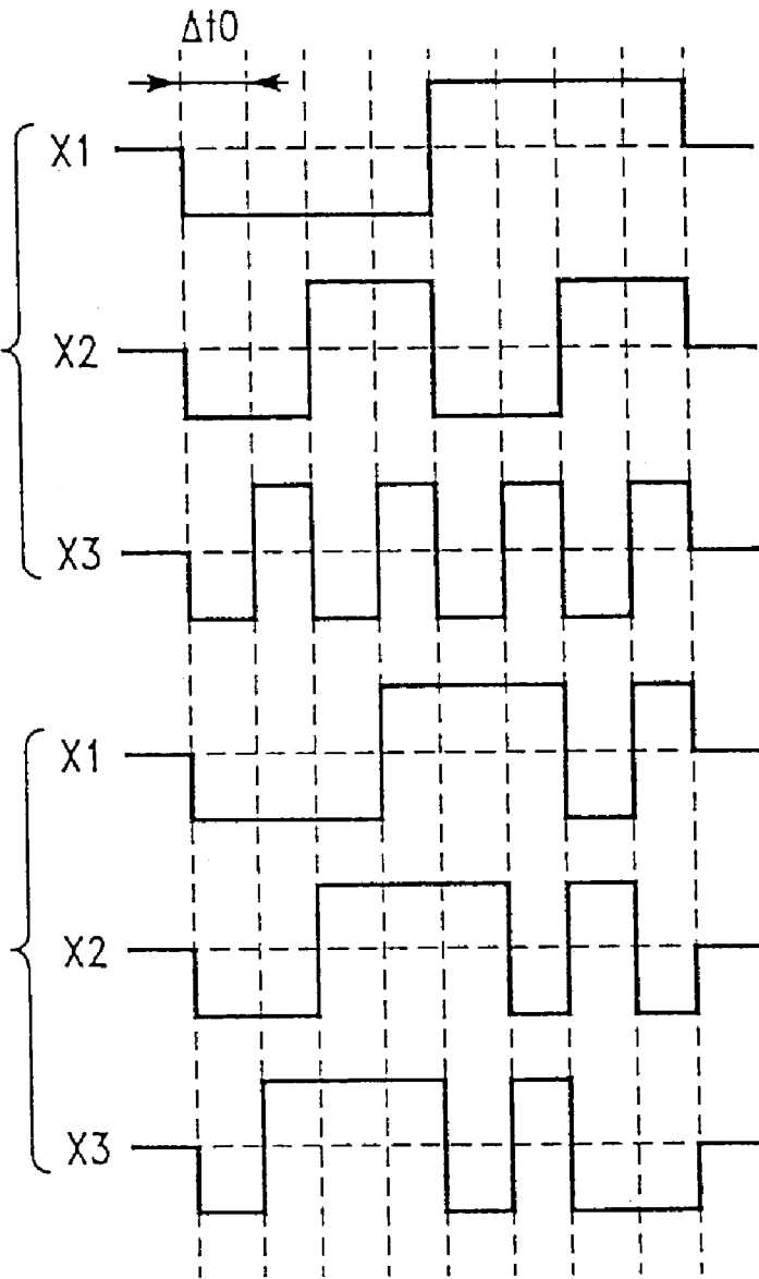
FIG.-46B (PRIOR ART)
