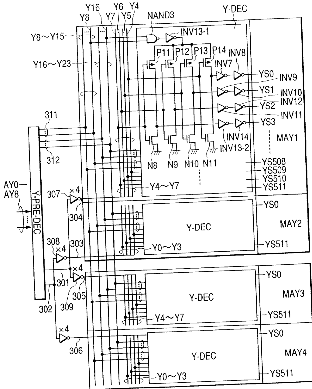
DETAILS OF Y-DECODER
