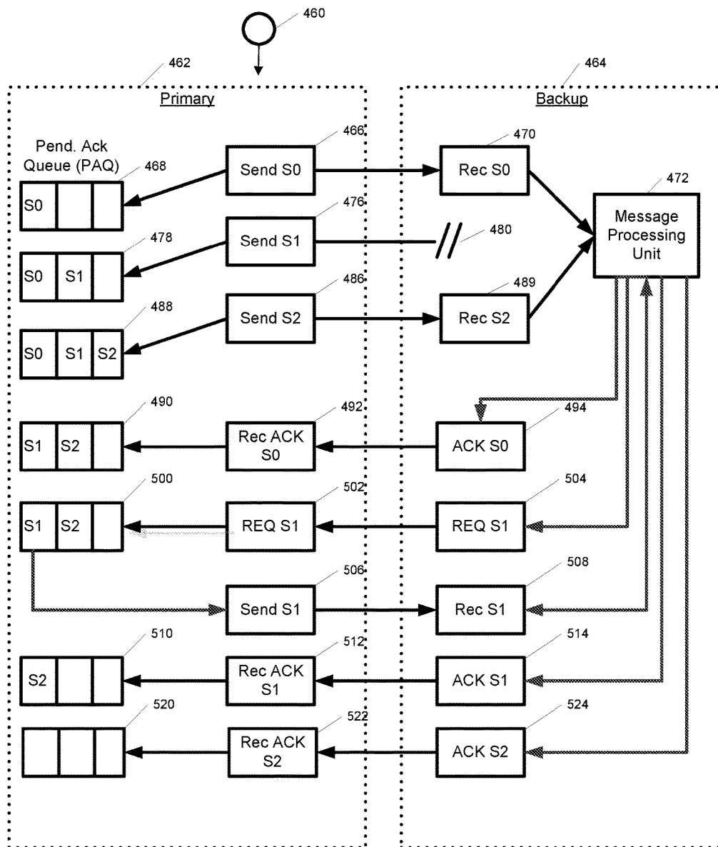
FIG. 12 – Multiple message with Retransmit
