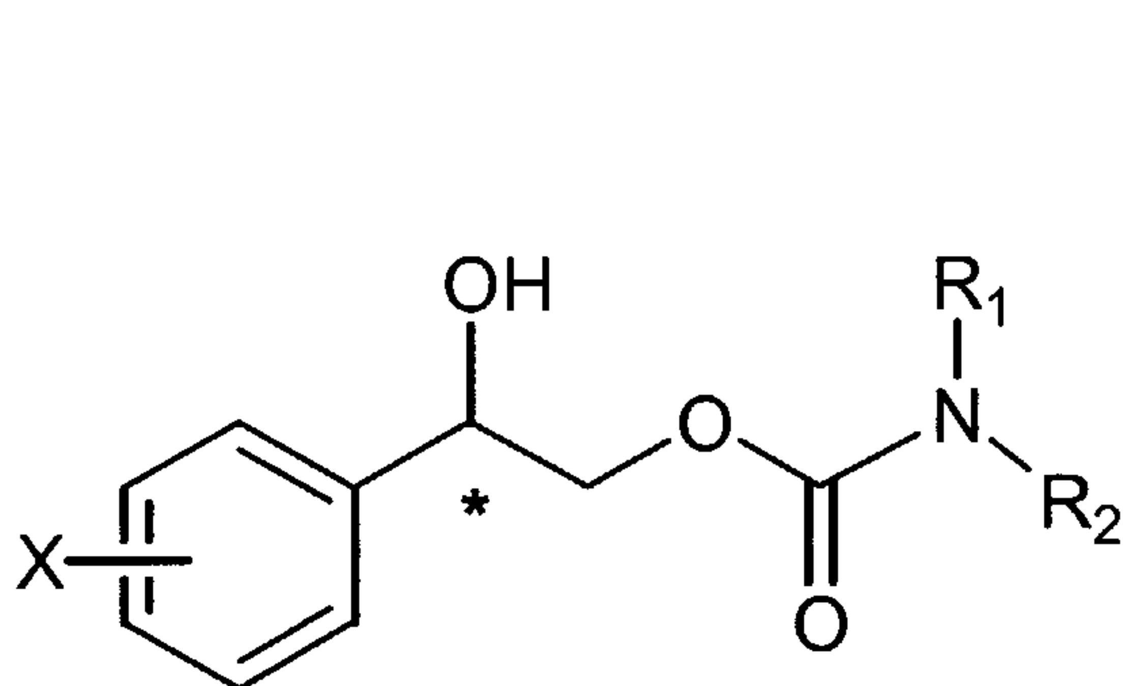
Formula (I)
