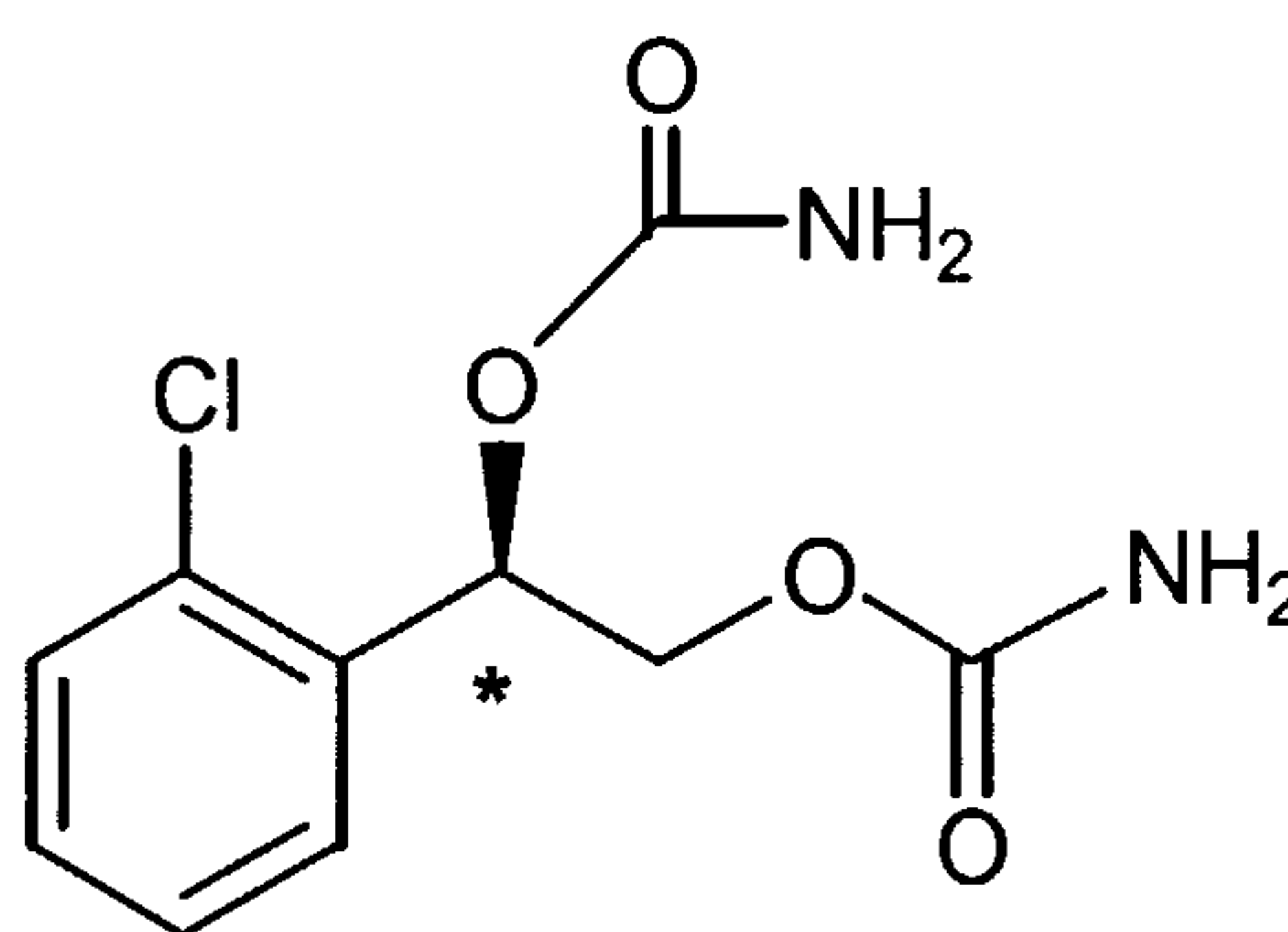
Formula (IIb)
