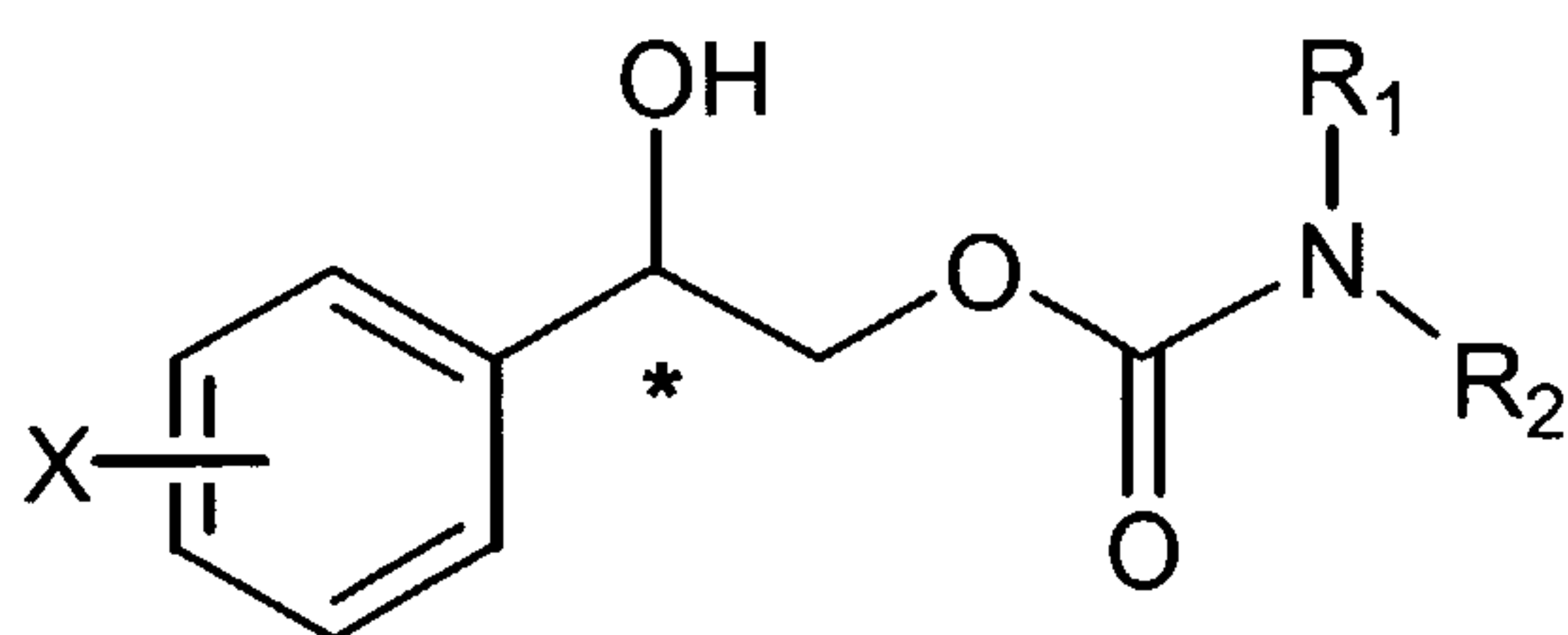
Formula (I)
