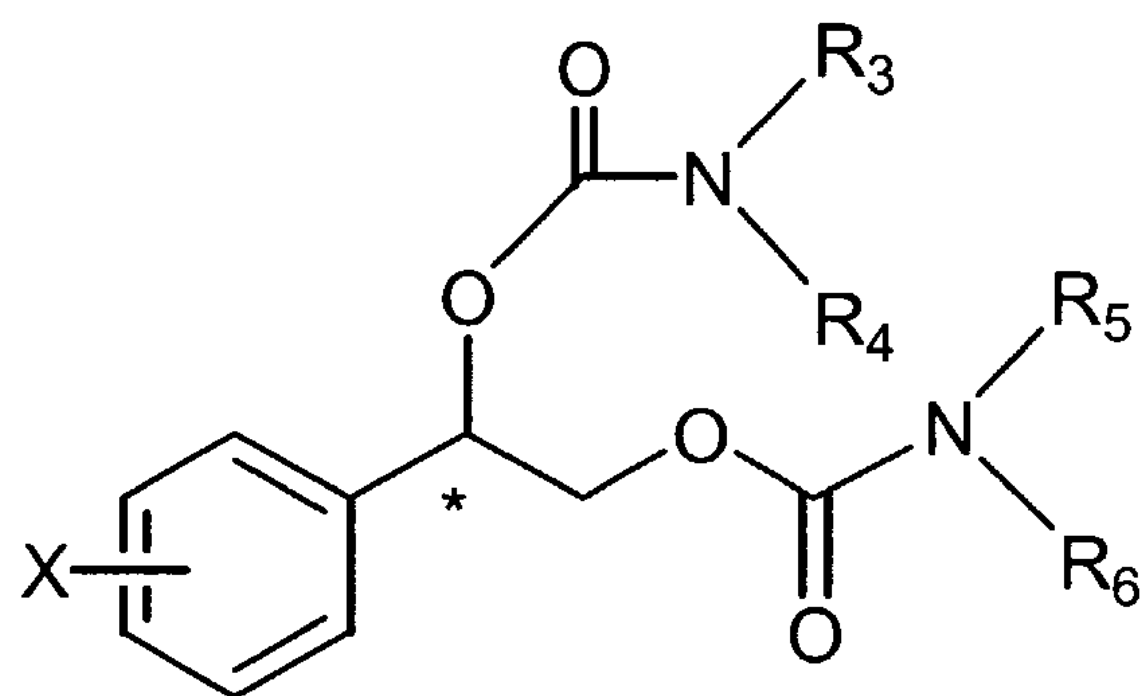
Formula (II)
