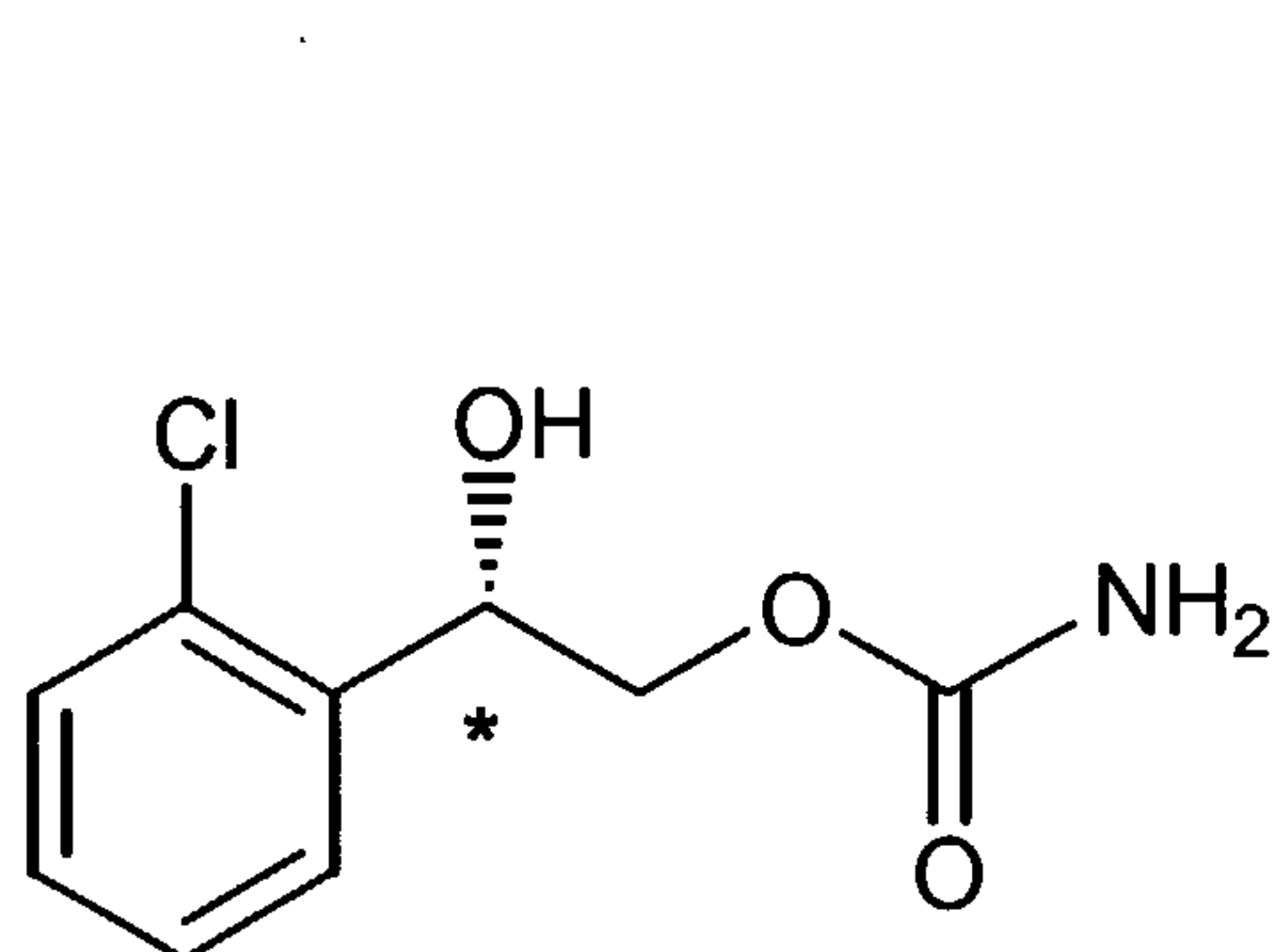
Formula (Ib)
