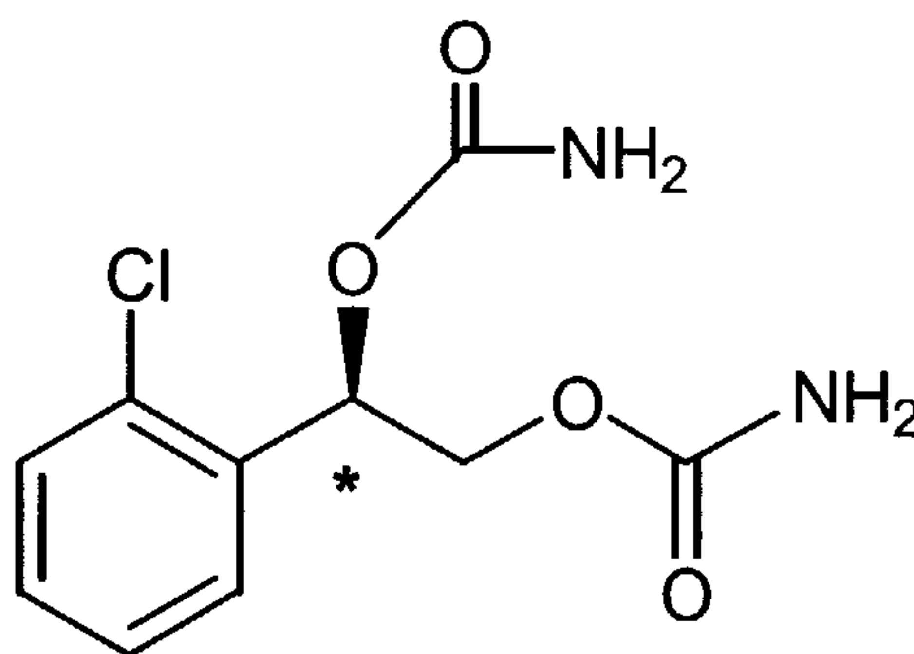
Formula (IIb)
