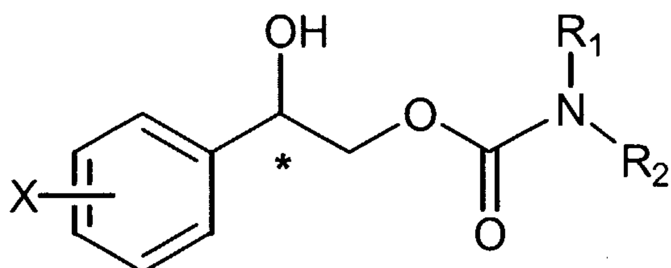
Formula (I)
