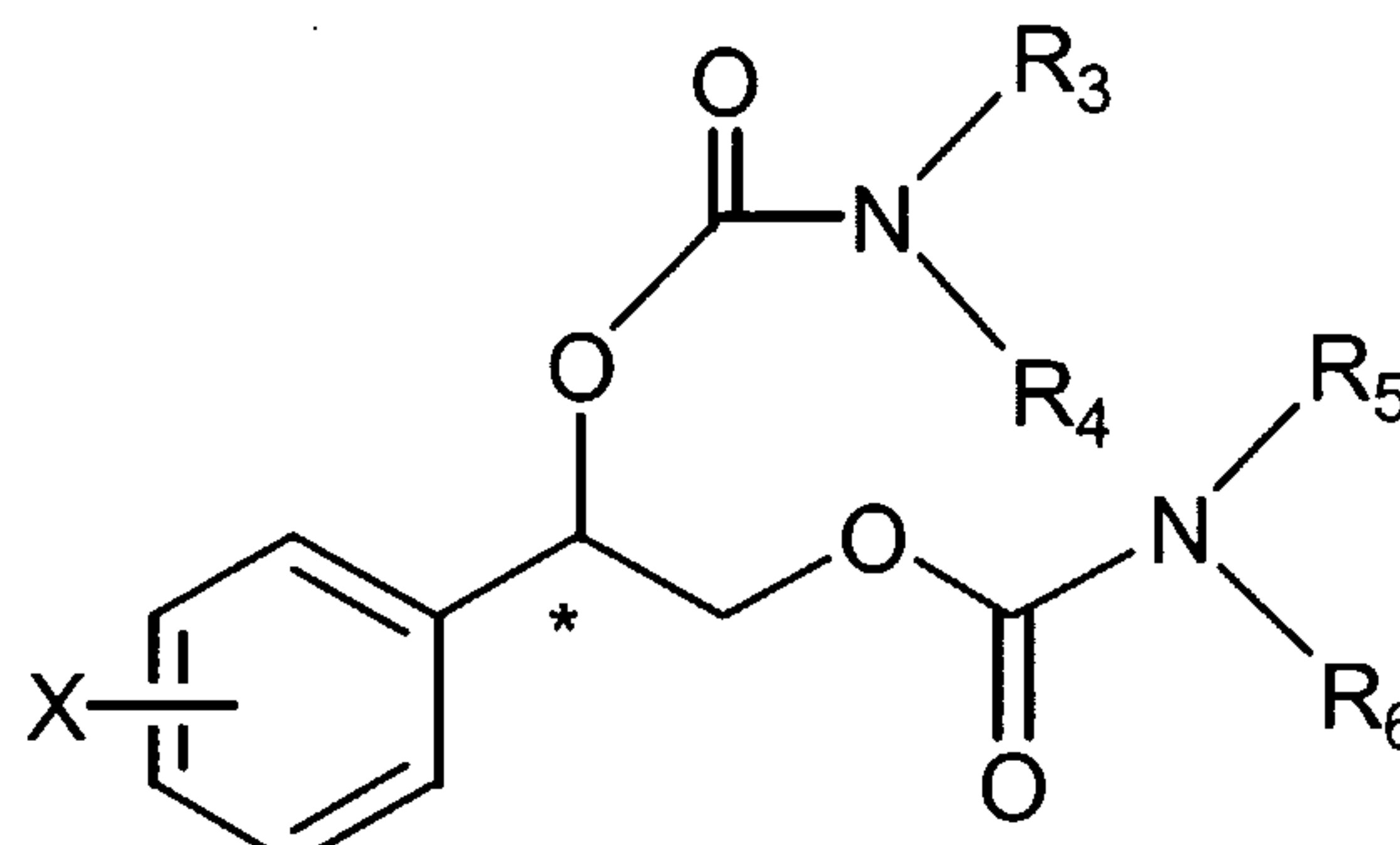
Formula (II)
