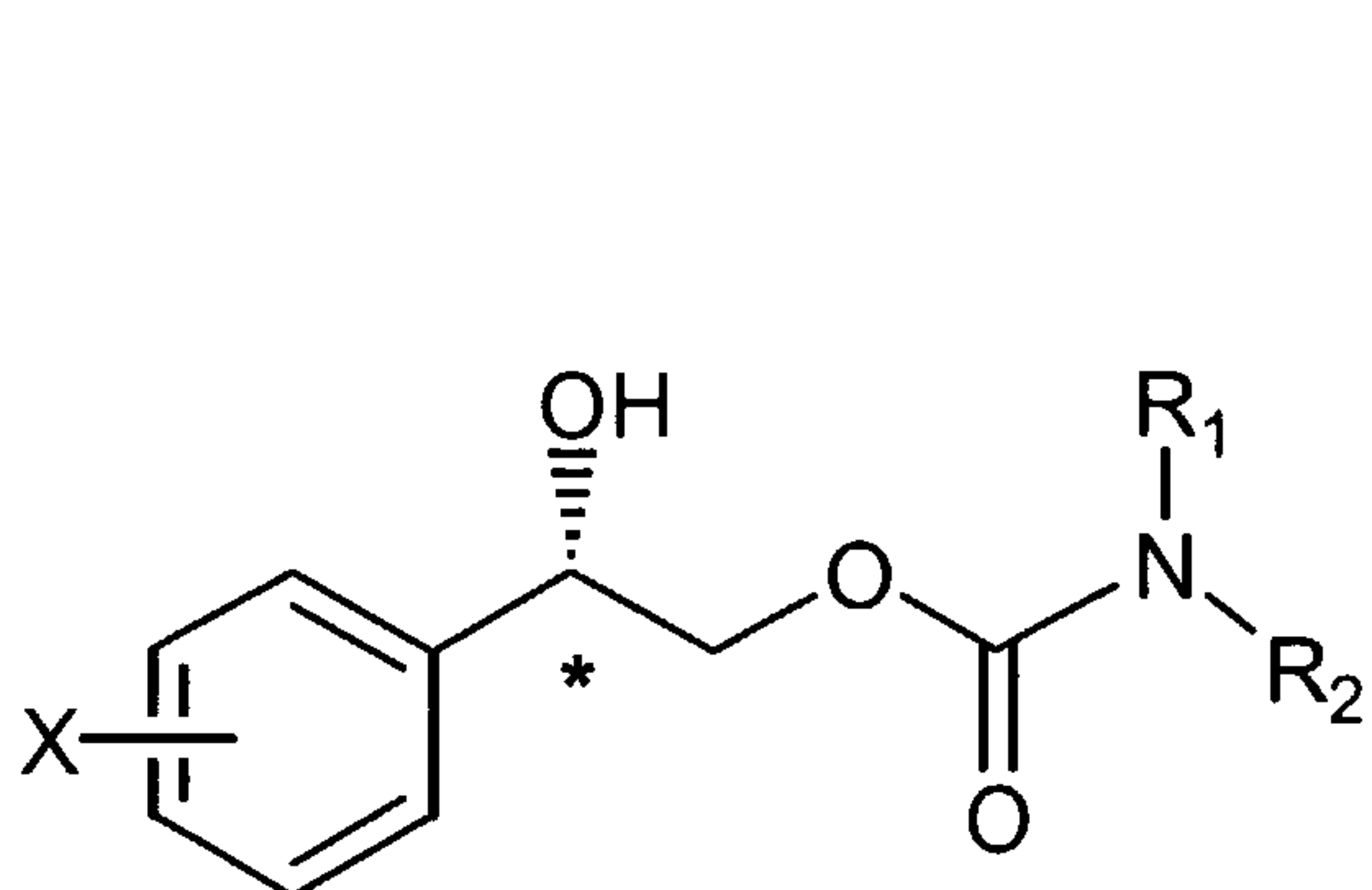
Formula (Ia)
