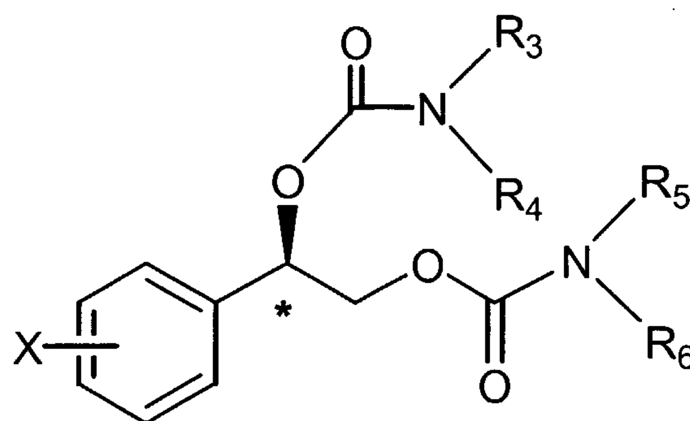
Formula (IIa)
