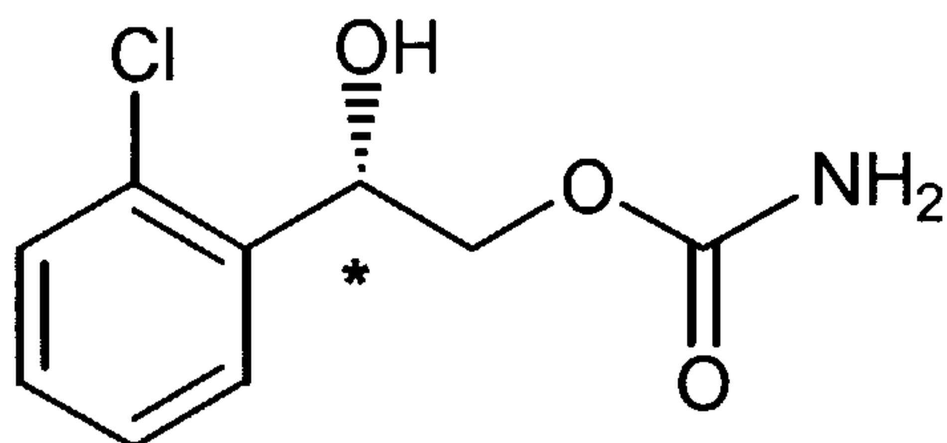
Formula (Ib)
