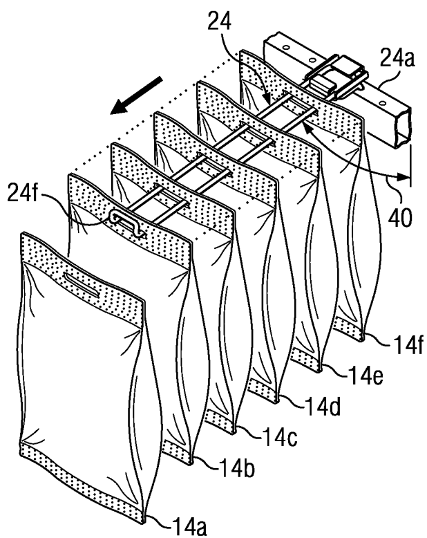
FIG. 3 (PRIOR ART)
