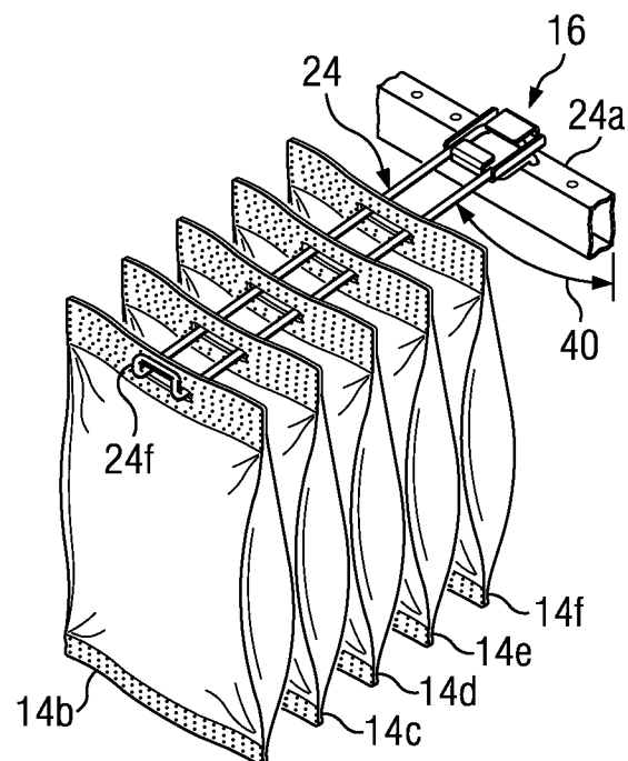
FIG. 4 (PRIOR ART)
