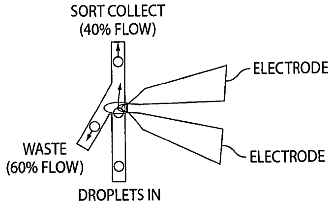
INVERTED FLUIDIC GEOMETRY (ASYMMETRIC FLOW GEOMETRY)
