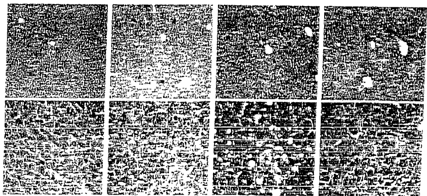
FIG - 13E 0 0.2 1 5 Tetracycline (mg/ml)
