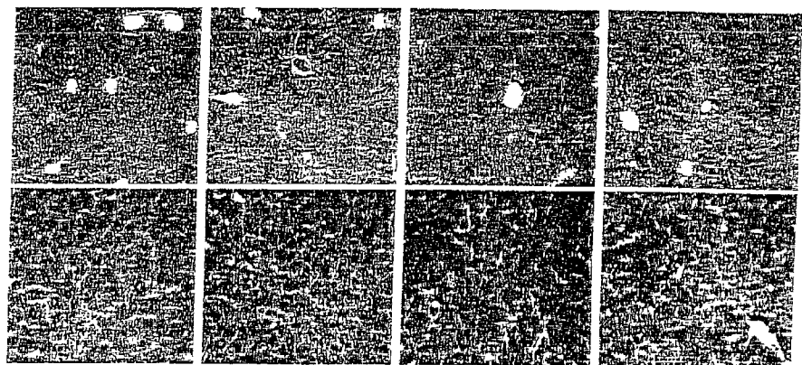
FIG - 13D 0 0.2 1 5 Tetracycline (mg/ml)
