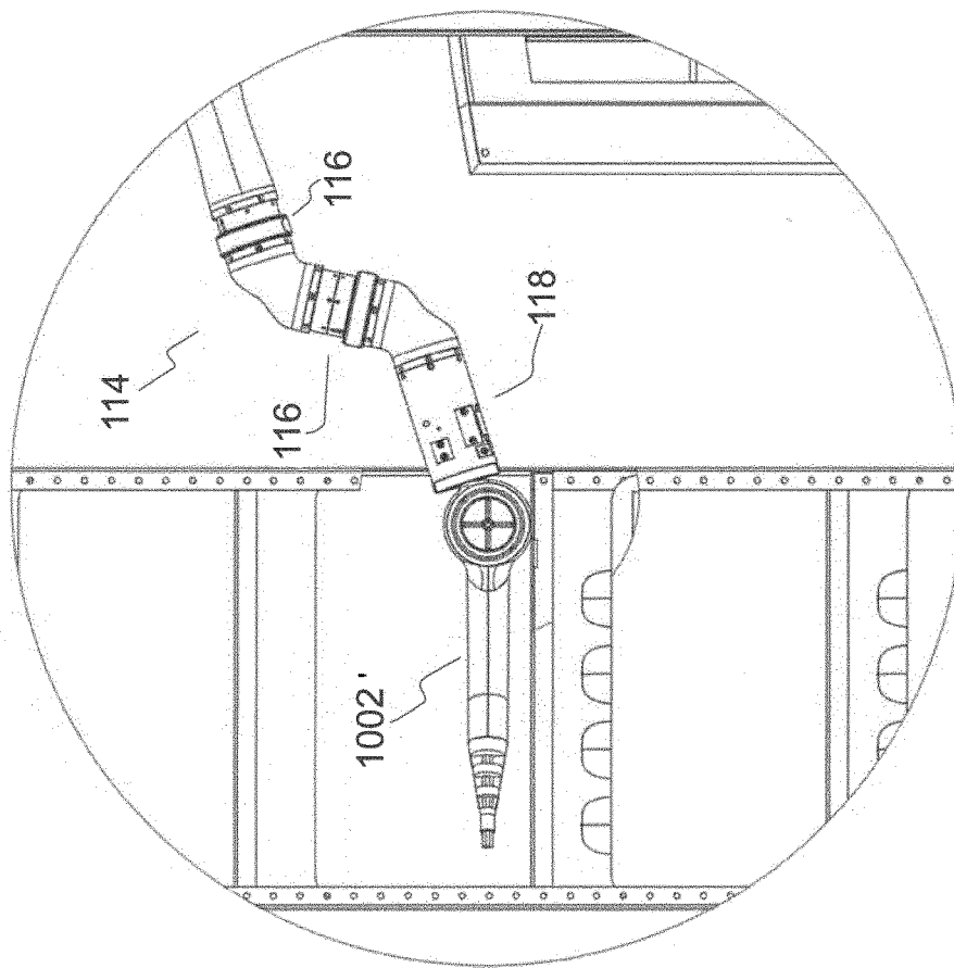
Fig. 24 DETAIL A
