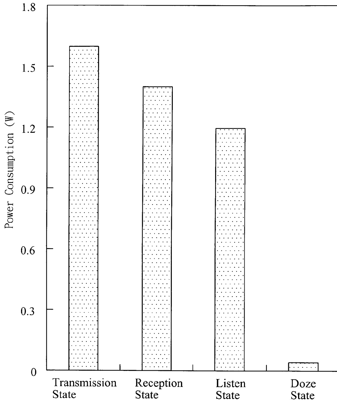
FIG. 2 (RELATED ART)
