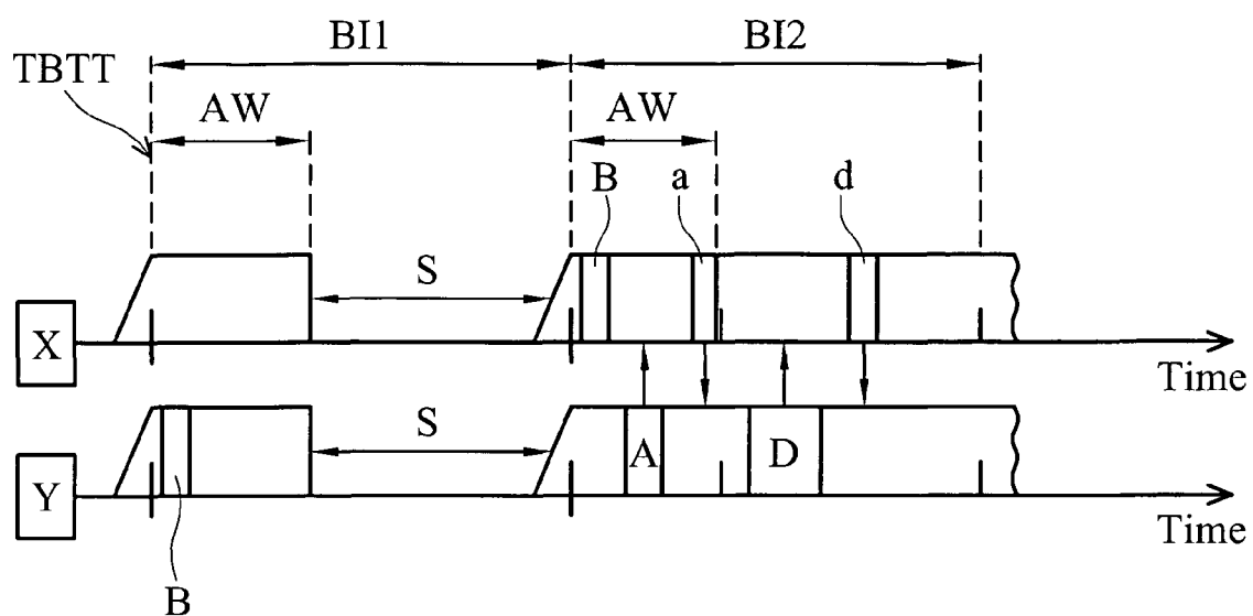
FIG. 3 (RELATED ART)
