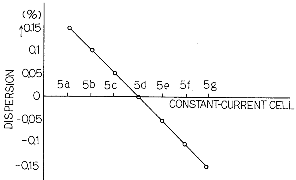
Fig.3 PRIOR ART
