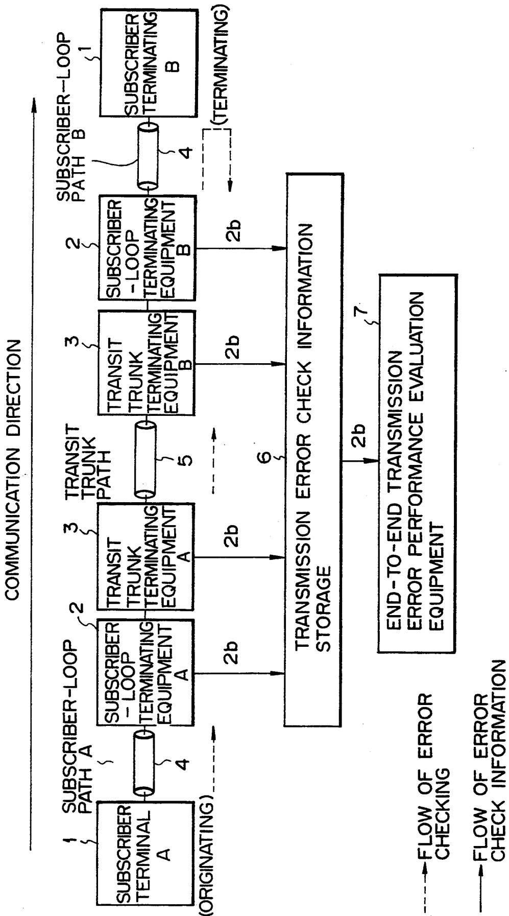
Fig. 2 PRIOR ART
