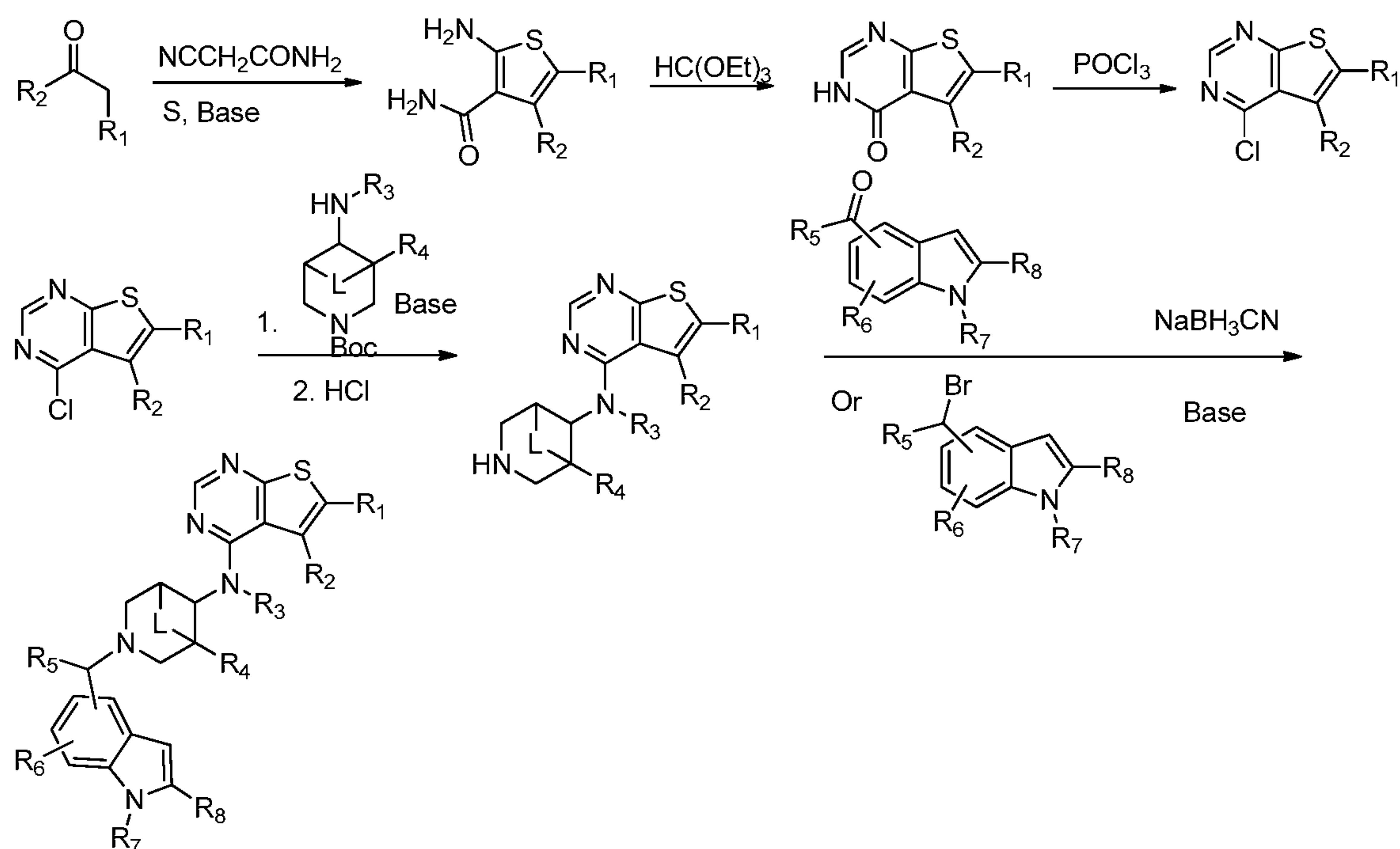
Scheme 7.
