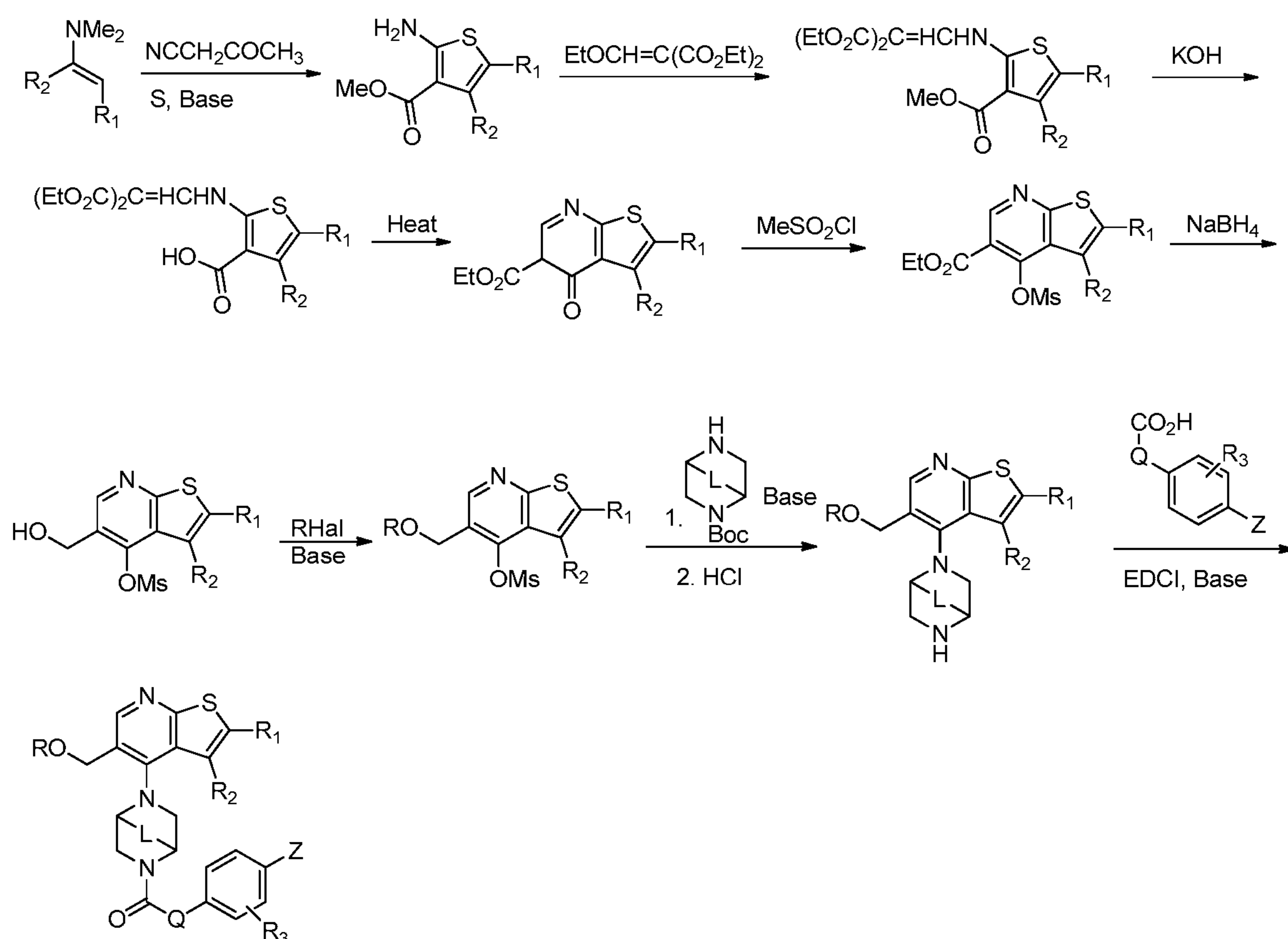
Scheme 4.
