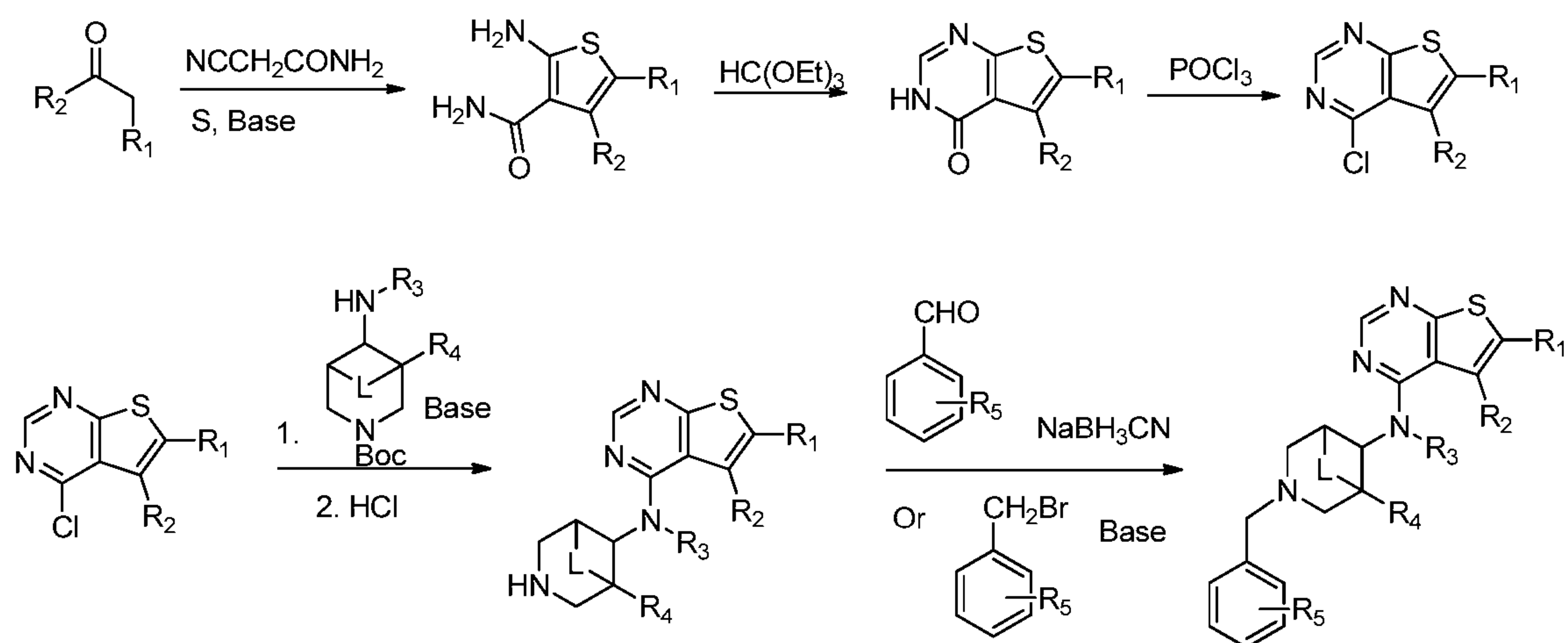
Scheme 5.
