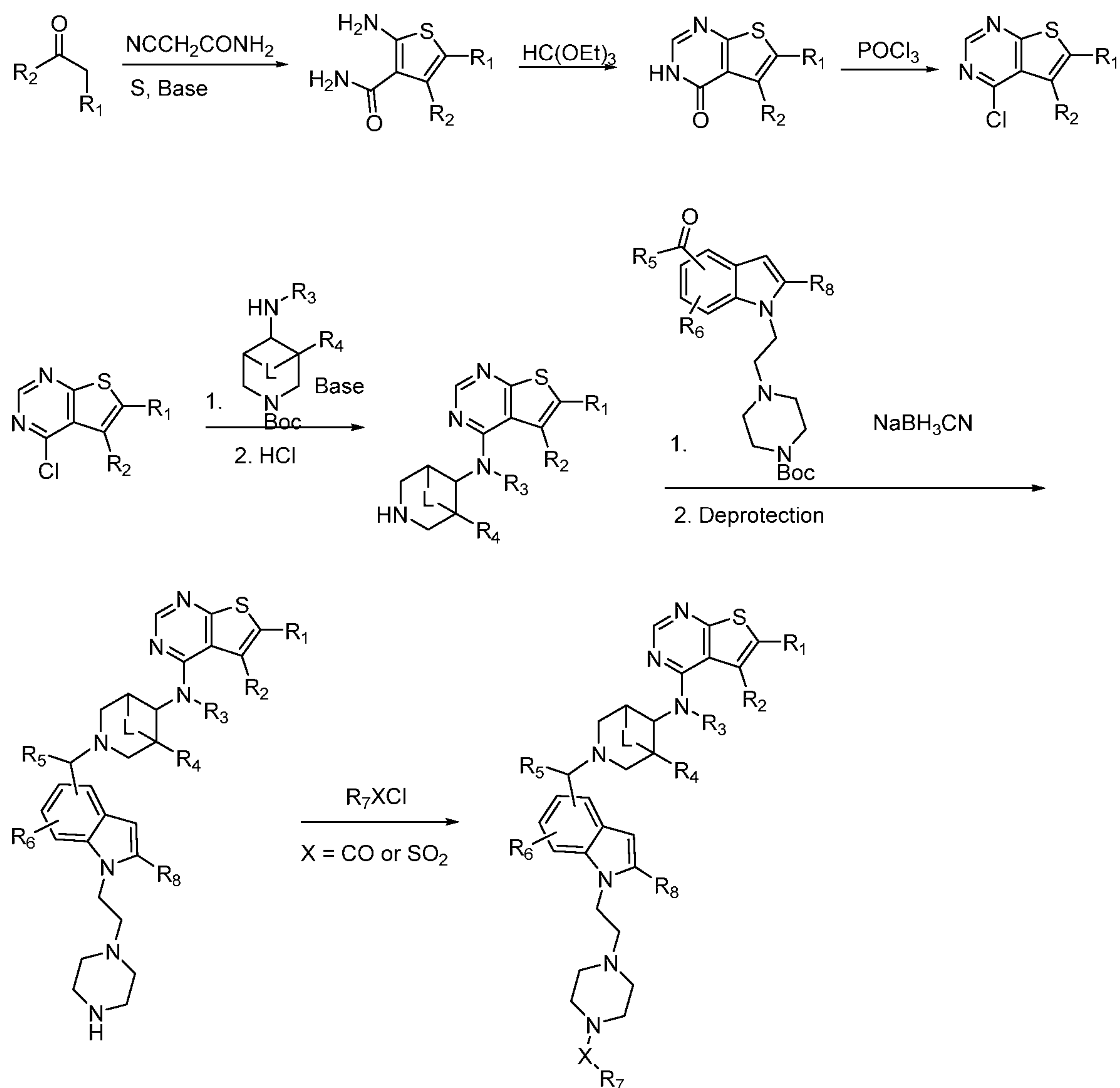
Scheme 9.
