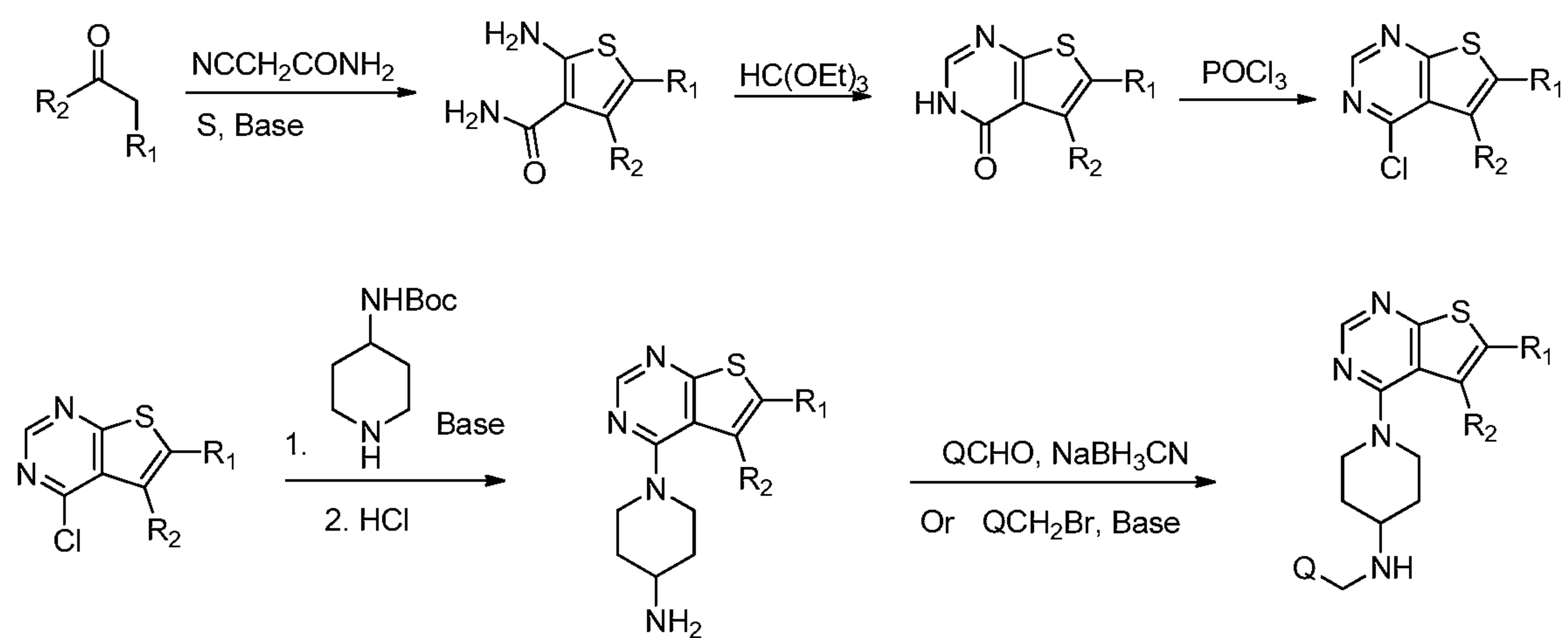
Scheme 12.
