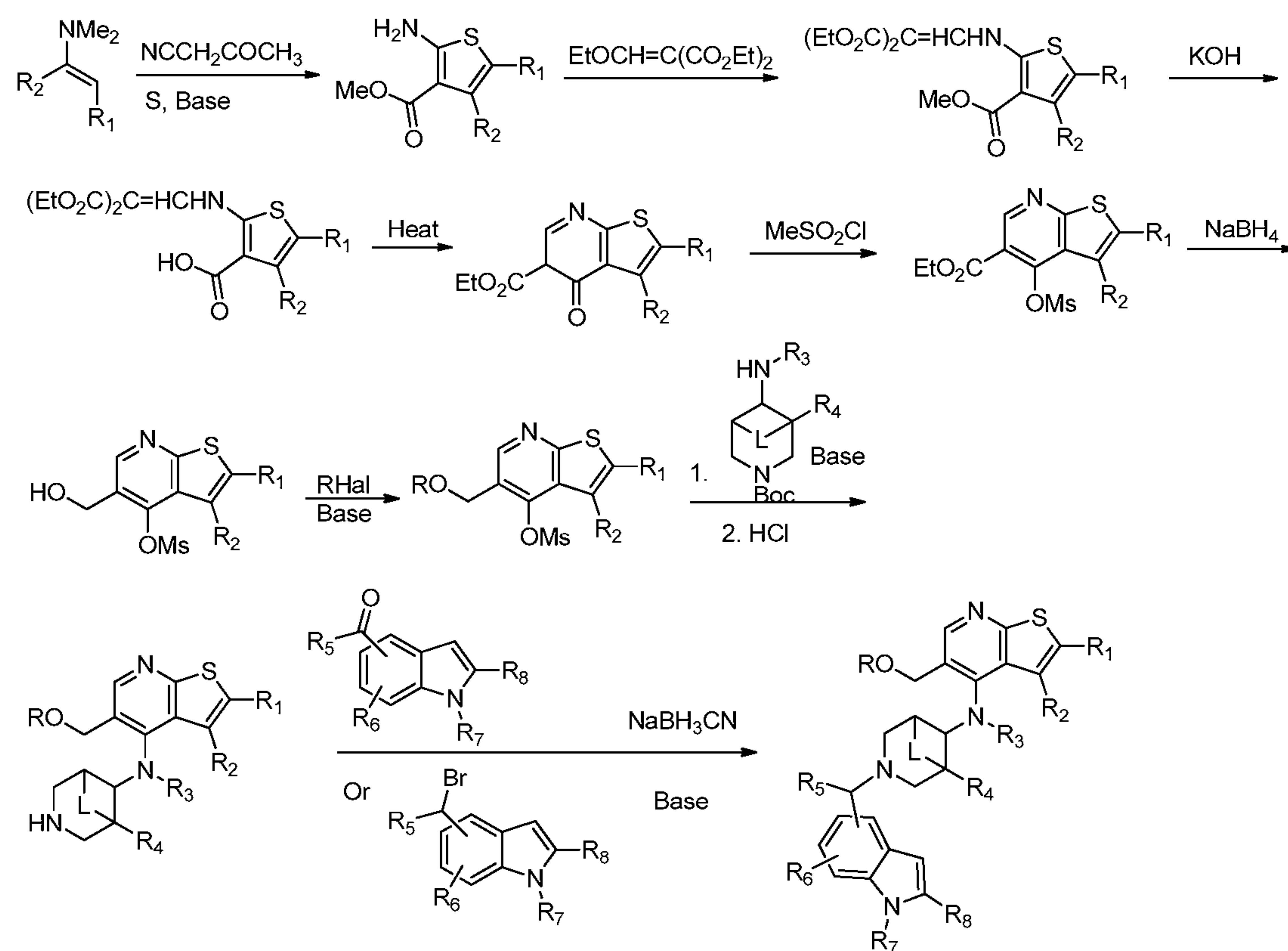
Scheme 8.
