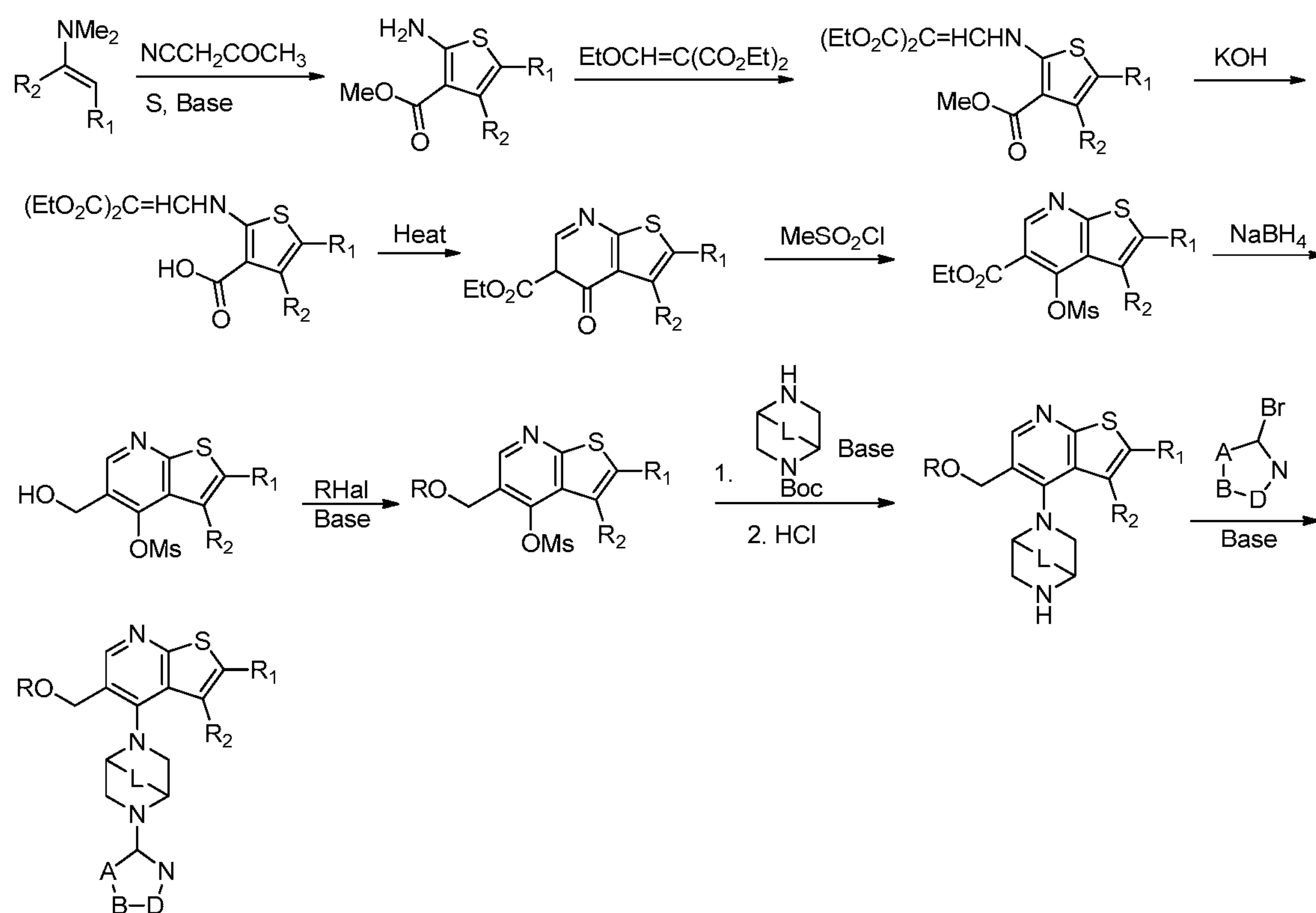
Scheme 2.
