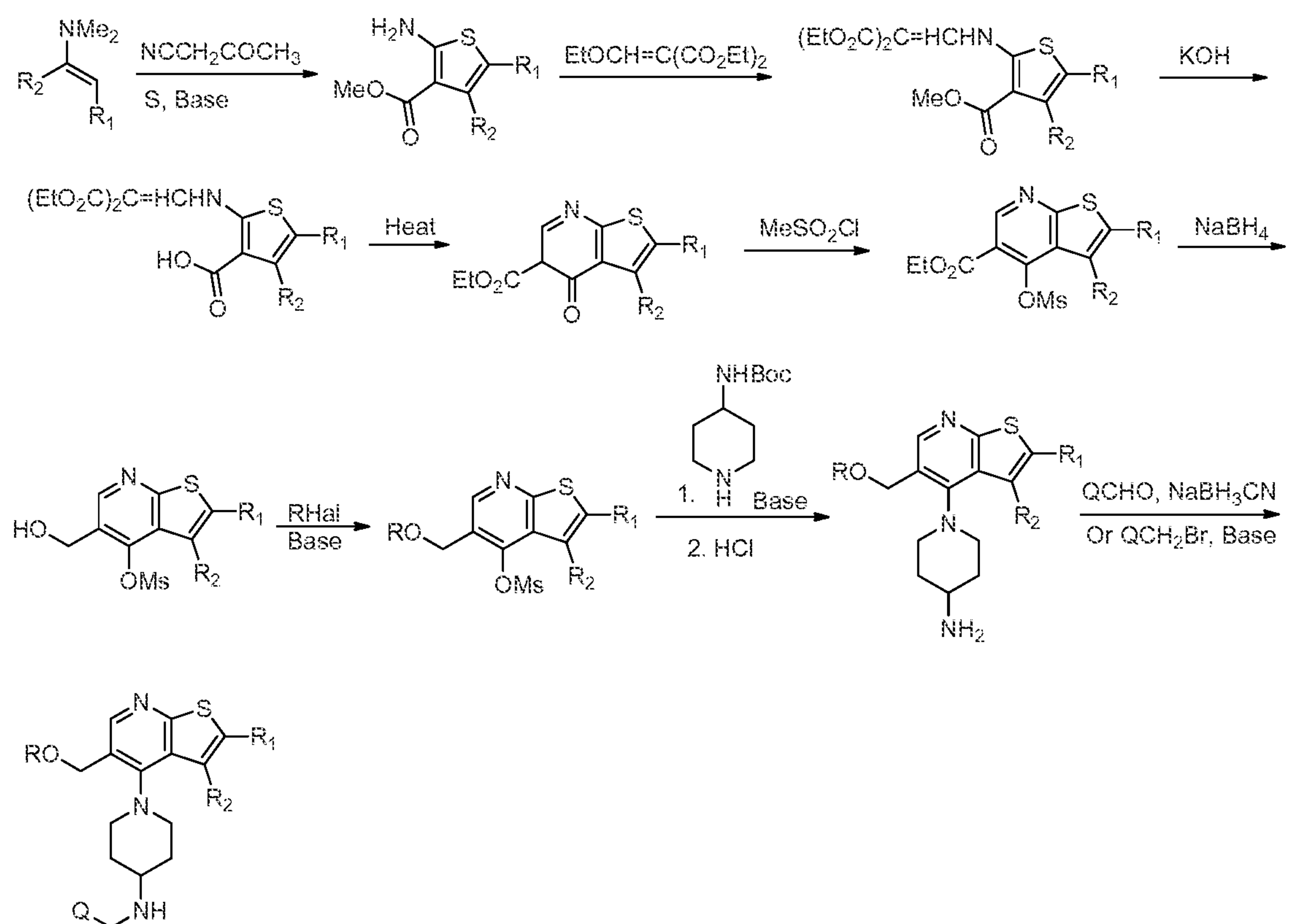
Scheme 13.
