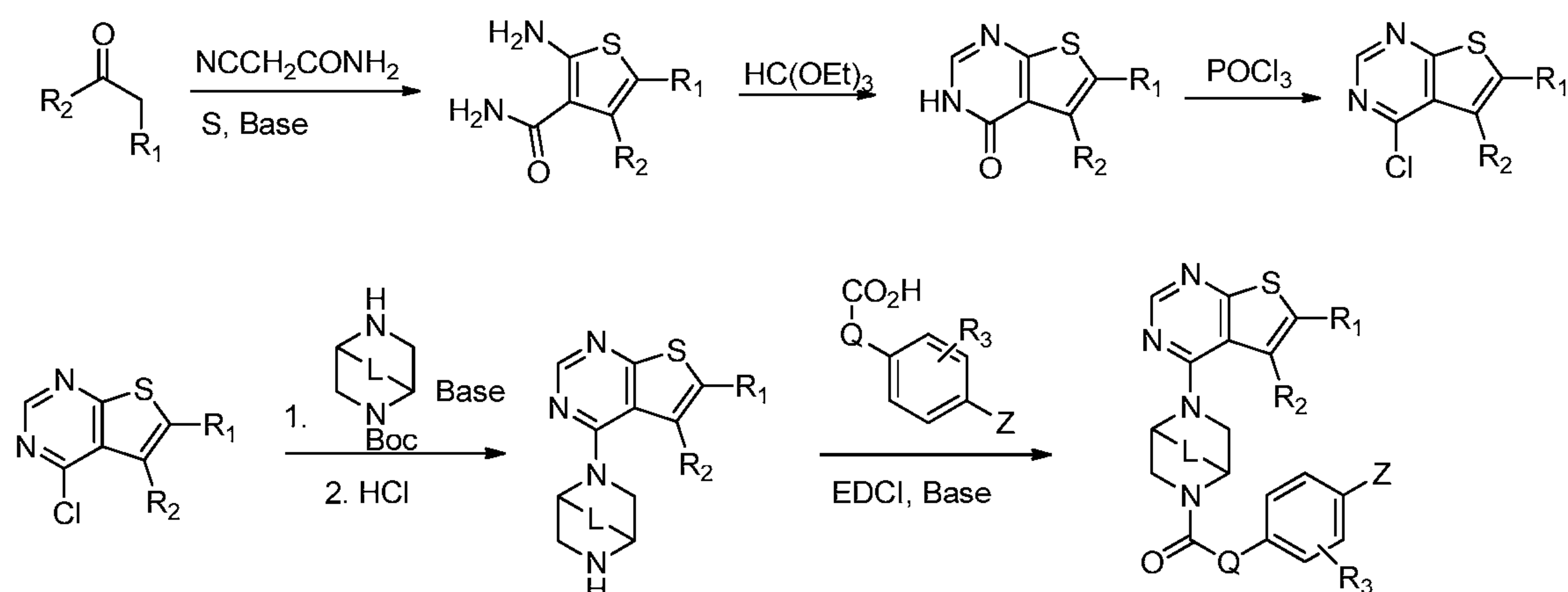
Scheme 4.
