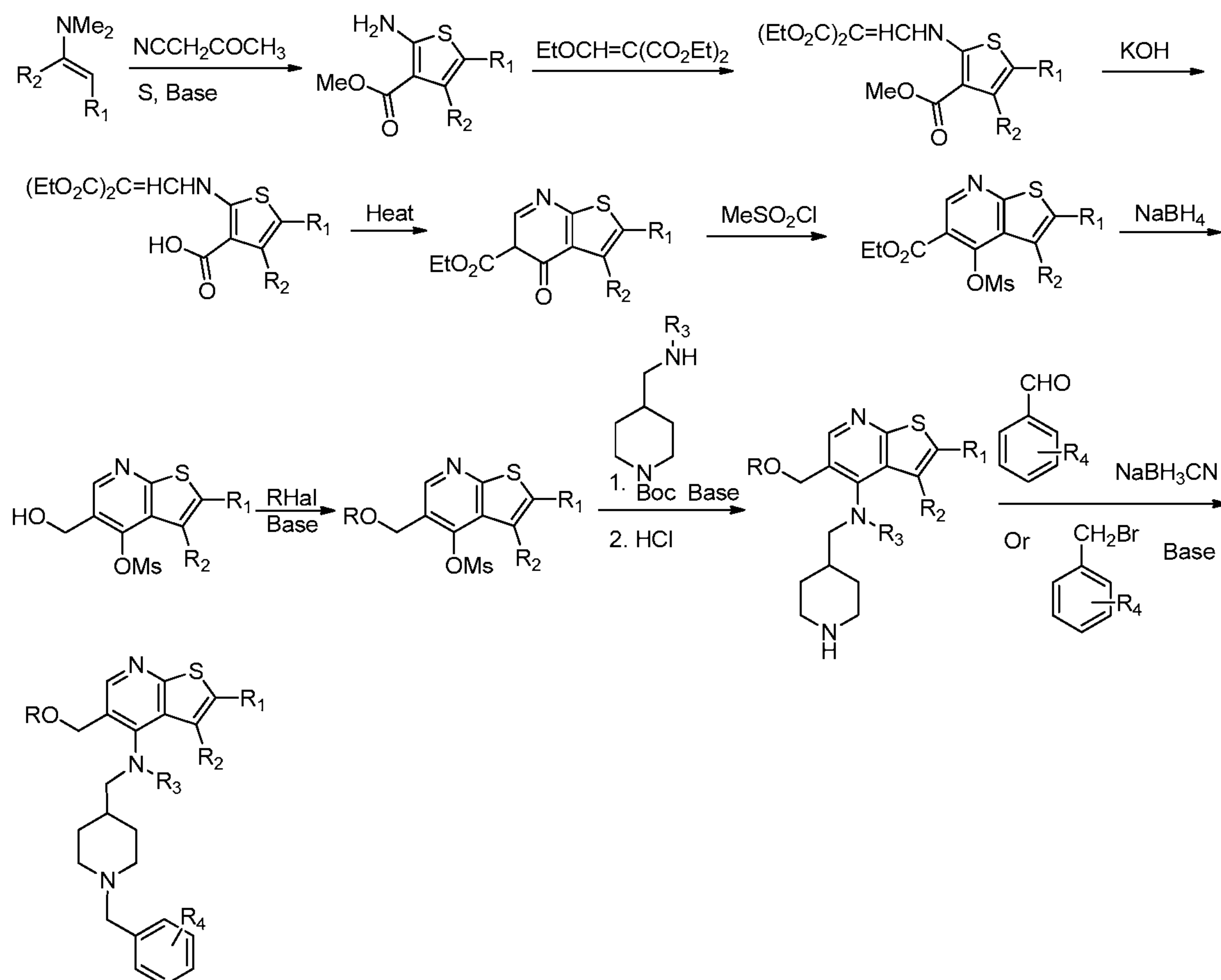
Scheme 11.
