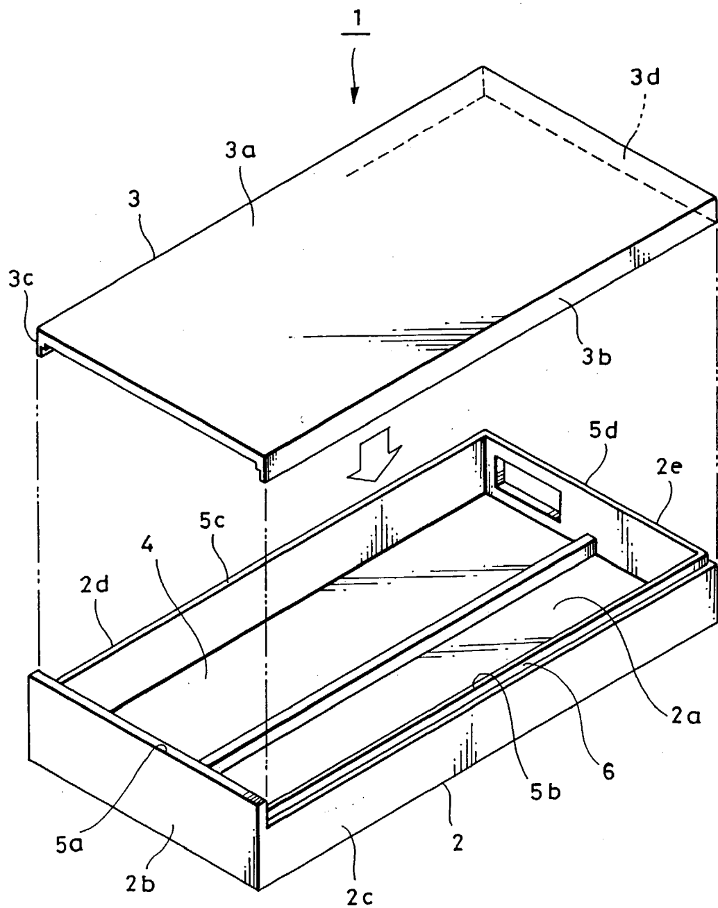
FIG. 8 ( PRIOR ART )
